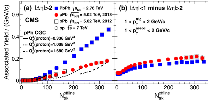
Fig. 6. Associated event-normalized yields for the near-side correlation function as a function of multiplicity N_{\text{trk}}^{\text{offline}} for 1 < p_T^{\text{trig}} < 2 GeV/c and 1 < p_T^{\text{assoc}} < 2 GeV/c under the same conditions as in Fig. 5. The results for 7 TeV pp collisions (open circles) [38] and 5.02 TeV pPb collisions from 2012 run (open squares) [34], as well as calculations from the Color Glass Condensate (CGC) theory (curves) [58], are also shown.
