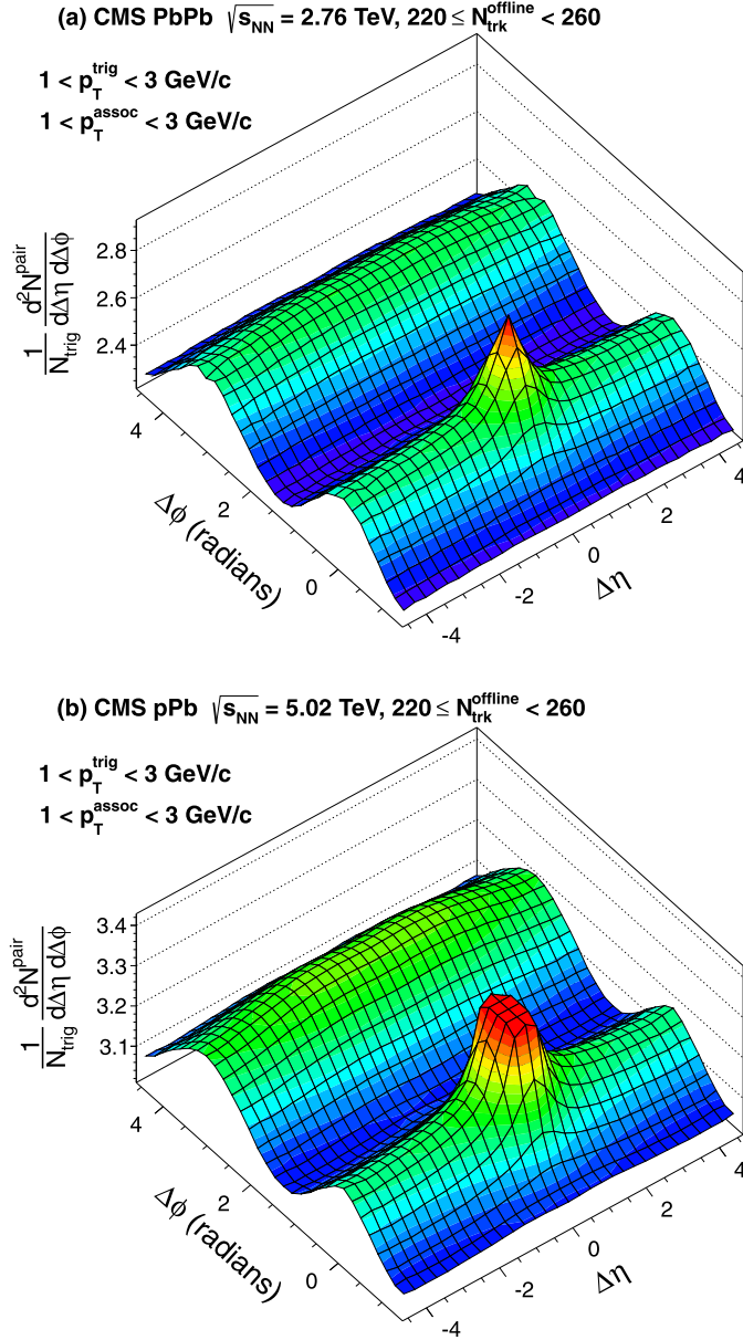
Fig. 2. The 2D two-particle correlation functions for (a) 2.76 TeV PbPb and (b) 5.02 TeV pPb collisions for pairs of charged particles with 1 < p_T^{trig} < 3 GeV/c and 1 < p_T^{assoc} < 3 GeV/c within the 220 \leq N_{trk}^{offline} < 260 multiplicity bin. The sharp near-side peak from jet correlations is truncated to emphasize the structure outside that region.
