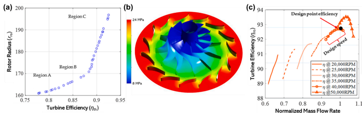
Fig. 10. ANN modelled supercritical CO 2 turbine efficiencies. (a) Optimized efficiencies for a range of rotor radii calculated from a multi-objective genetic algorithm optimization of an ANN model. (b) Multiphysics simulation of pressure distribution of the on the surface of the optimized hub/rotor geometry. (c) Simulated off-design performance of the optimized turbine geometry.
