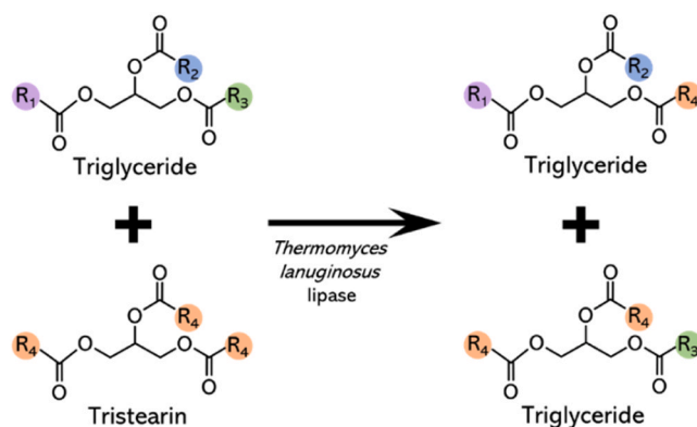
Fig. 7. Reaction mechanism between triglycerides and tristearin during supercritical enzymatic transesterification. Either of the fatty acids, R 1 and R 3 , are liberated by the thermomyces lanuginosus lipase as well as a steric acid from tristearin and exchanged leading to the formation of different triglycerides.
