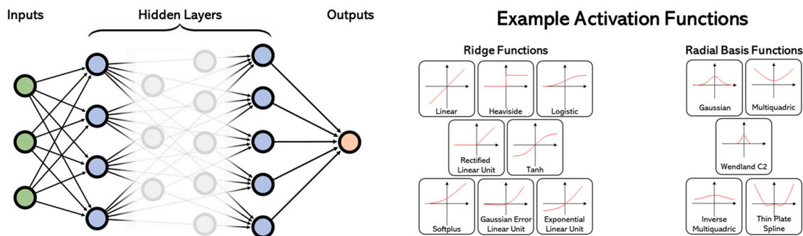
Fig. 3. Typical representation of an artificial neural network (ANN). A given set of inputs (green circles) are fed into a network of nodes organized in layers (blue circles) before calculating an output (orange circle). Each node within the hidden layer represents a mathematical 'activation' function. Typically, these are either ridge or radial basis functions. Examples of activation functions are given to the right of the main diagram. The exact forms and weights used in the functions within the hidden layers are determined during training.
