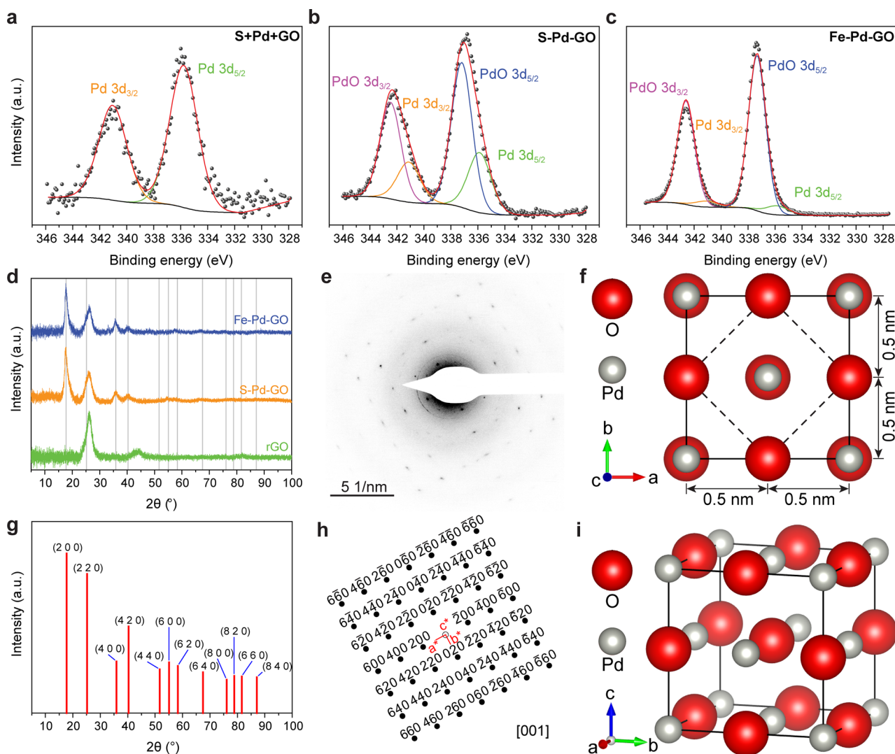
Figure 3. Composition and proposed structure of the nanofilm. High-resolution Pd 3d XPS of (a) S+Pd+GO, the precursor of S-Pd-GO before the hydrothermal process, (b) S-Pd-GO, and (c) Fe-Pd-GO. (d) XRD of S-Pd-GO and Fe-Pd-GO. The vertical gray lines indicate the peak position from the XRD simulation in (g). (e) SAED of the nanofilm. (f) Proposed structure of PdO square network in [001] projection with a = b = 1 nm (solid line) or a = b = \sqrt{2}/2 nm (dashed line). Simulated (g) XRD and (h) SAED from the structure in (f). Only XRD and SAED patterns from hk0 are presented due to the nature of the thin nanofilm. (i) One of several proposed unit cells of PdO with face-centered cubic structure ( a = b = c = 1 nm).
