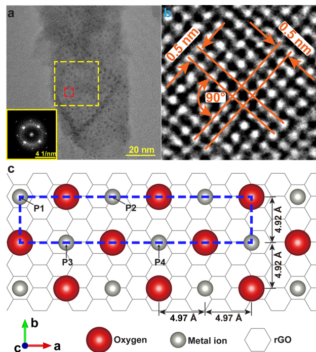
Figure 4. Morphology of Fe–Ag–GO and proposed model of lattice-matching between metal oxides and rGO. (a) TEM of Fe–Ag–GO. Inset: FFT of the yellow square area in (a). (b) HRTEM of the red square area in (a). (c) Metal ions and oxygen are in four positions (P1–P4) of the rGO lattice. The blue box indicates a repeating unit.
