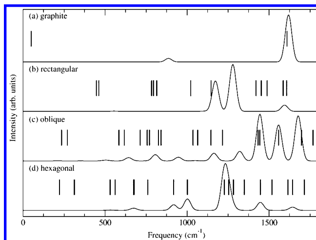
Figure 3. Simulated infrared absorption spectra for graphite (a) and Haeckelite planar structures (b), (c), (d): (b) rectangular ( R_{5,7} ), (c) oblique ( O_{5,6,7} ), (d) hexagonal ( H_{5,6,7} ). The Raman frequencies (vertical lines) are also given.
