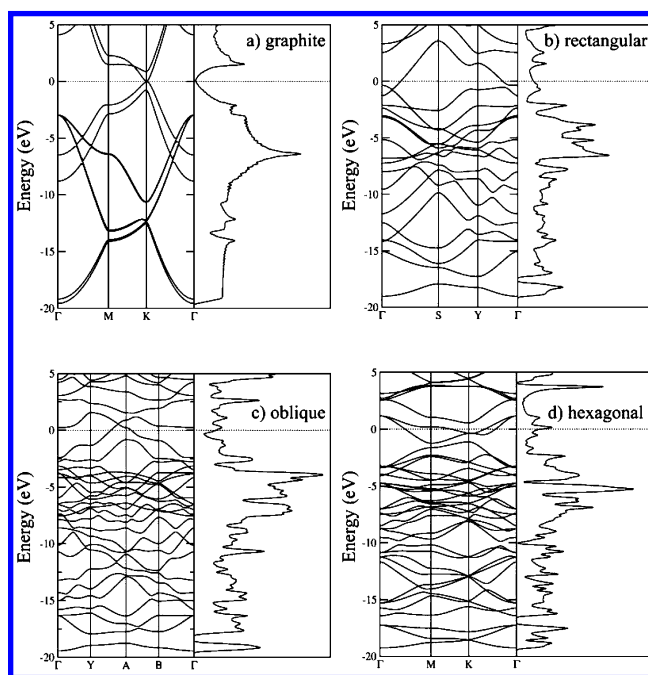
Figure 2. Band structure and electronic density of states (Fermi level positioned at zero energy) for graphite exhibiting semimetallic behavior (a) and for Haeckelites (b), (c), (d) showing metallic behavior. (b) rectangular (R 5,7 ), (c) oblique (O 5,6,7 ), (d) hexagonal (H 5,6,7 ). In all plots, the units of the density of states are states per eV.
