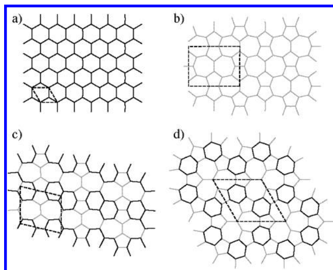
Figure 1. Schematic representation of four different layered sp^2 -like carbon atomic arrangements with their respective unit cell: (a) graphite, (b) rectangular ( R_{5,7} ), (c) oblique ( O_{5,6,7} ), (d) hexagonal ( H_{5,6,7} ). The six-membered rings are highlighted.
