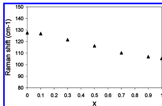
Figure 5. Evolution of a Raman shift ( \text{cm}^{-1} ) vs the amount of tantalum in the (\text{Ta}_x\text{Nb}_{1-x})_2\text{O}_5 oxides.
