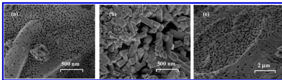
Figure 7. SEM images of the (a) (\text{Ta}_x\text{Nb}_{1-x})_2\text{O}_5 ( x = 0.9 ), (b) \text{Ta}_x\text{Nb}_{1-x}\text{VO}_5 ( x = 0.5 ), and (c) \text{Ta}_x\text{Nb}_{1-x}\text{BiO}_4 ( x = 0.5 ) mixed oxides.
