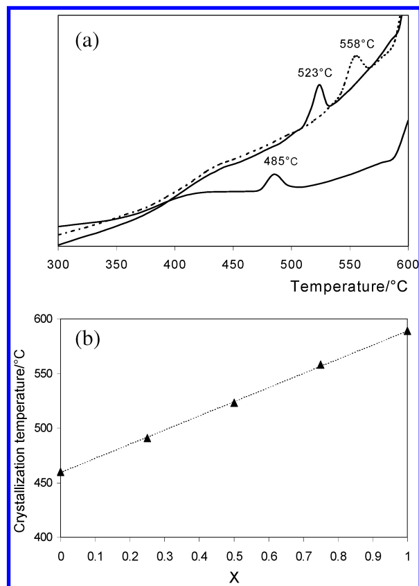
Figure 8. (a) DSC analysis of the \text{Ta}_x\text{Nb}_{1-x}\text{VO}_5 oxide precursors. (b) Evolution of the crystallization temperature with the amount of tantalum.
