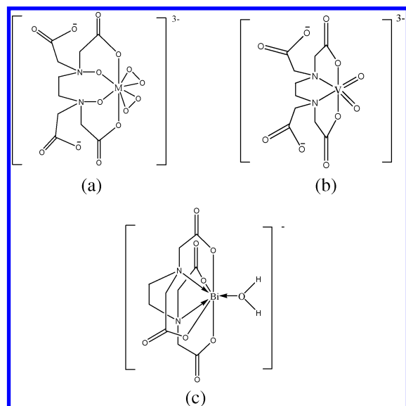
Figure 1. Chemical structures of the various anionic complexes used for the preparation of the mixed oxides: (a) [M(O_2)_2(EDTAO_2)]^{3-} ( M = Nb or Ta ), (b) [V(O)_2(EDTA)]^{3-} and [Bi(EDTA)(H_2O)]^- .
