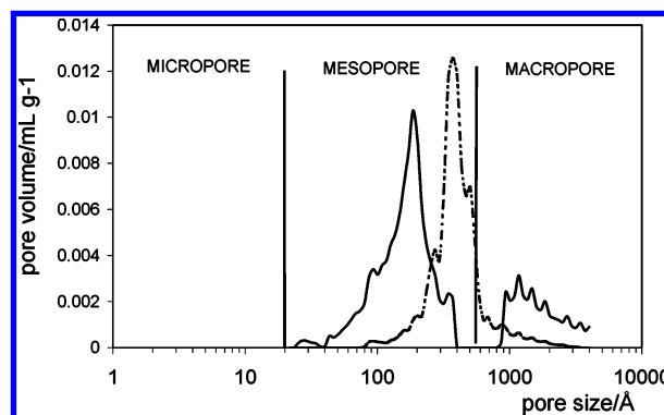
Figure 6. BJH pore-size distribution of the (\text{Ta}_x\text{Nb}_{1-x})_2\text{O}_5 mixed oxides with x = 0.5 (straight line) and x = 0.3 (dashed line).
