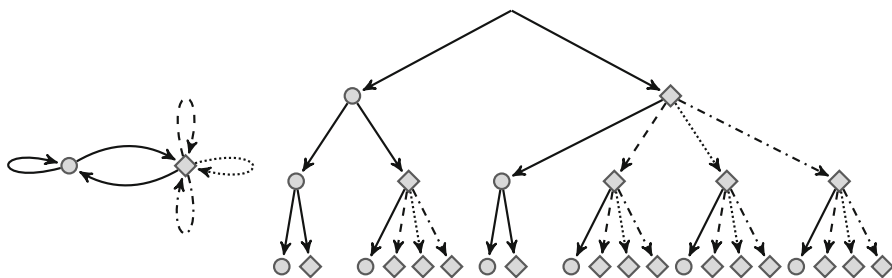
Fig. 2 Illustration of the tree constructed from the graph on the left
