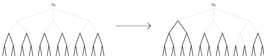
Fig. 1 The trees T_1 and T_2 are indicated with dotted lines
