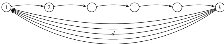
Fig. 3 Matui's graph g such that V_{d,k} = \mathcal{F}(\mathcal{G}_g)
