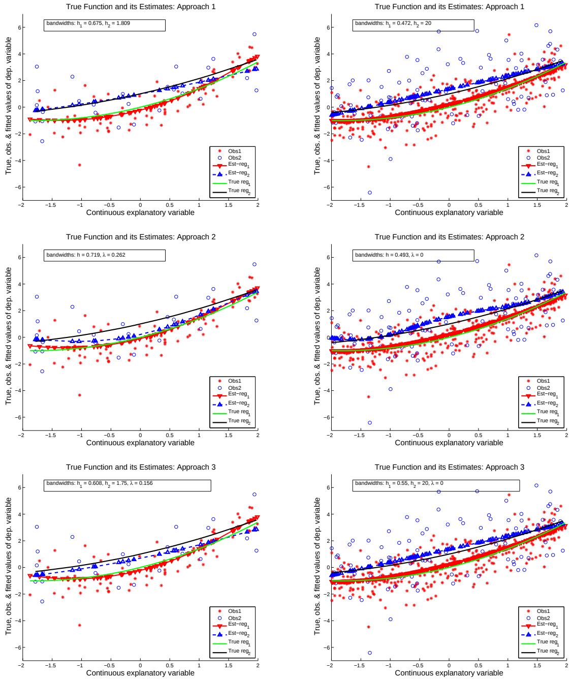
Figure 3: Example 4: Left panel, n = 100 and right panel, n = 400 . From top to bottom: Approach1 (no-smoothing the discrete variable), Approach2 (simple- smoothing), Approach3 (complete-smoothing).
