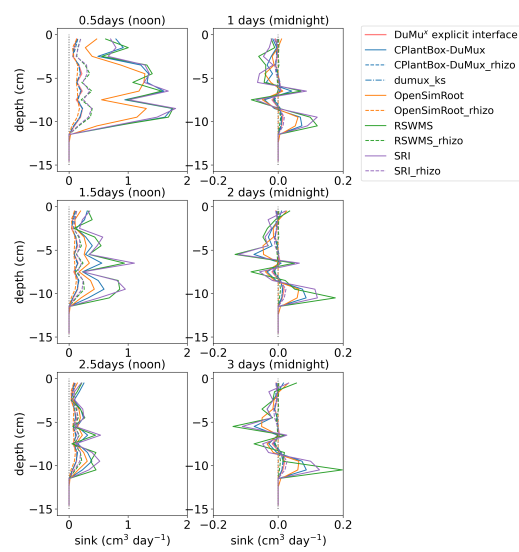
(a) Constant k_r and k_x
