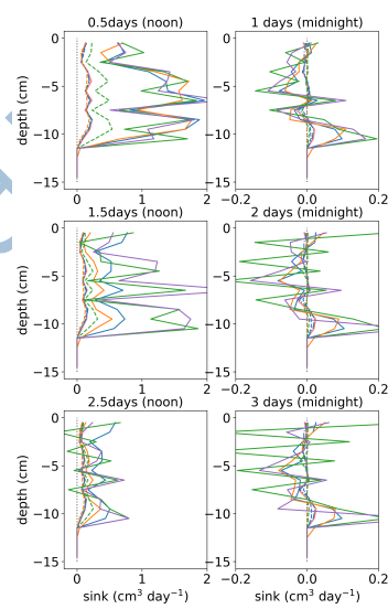
(b) Age-dependent k_r and k_x
