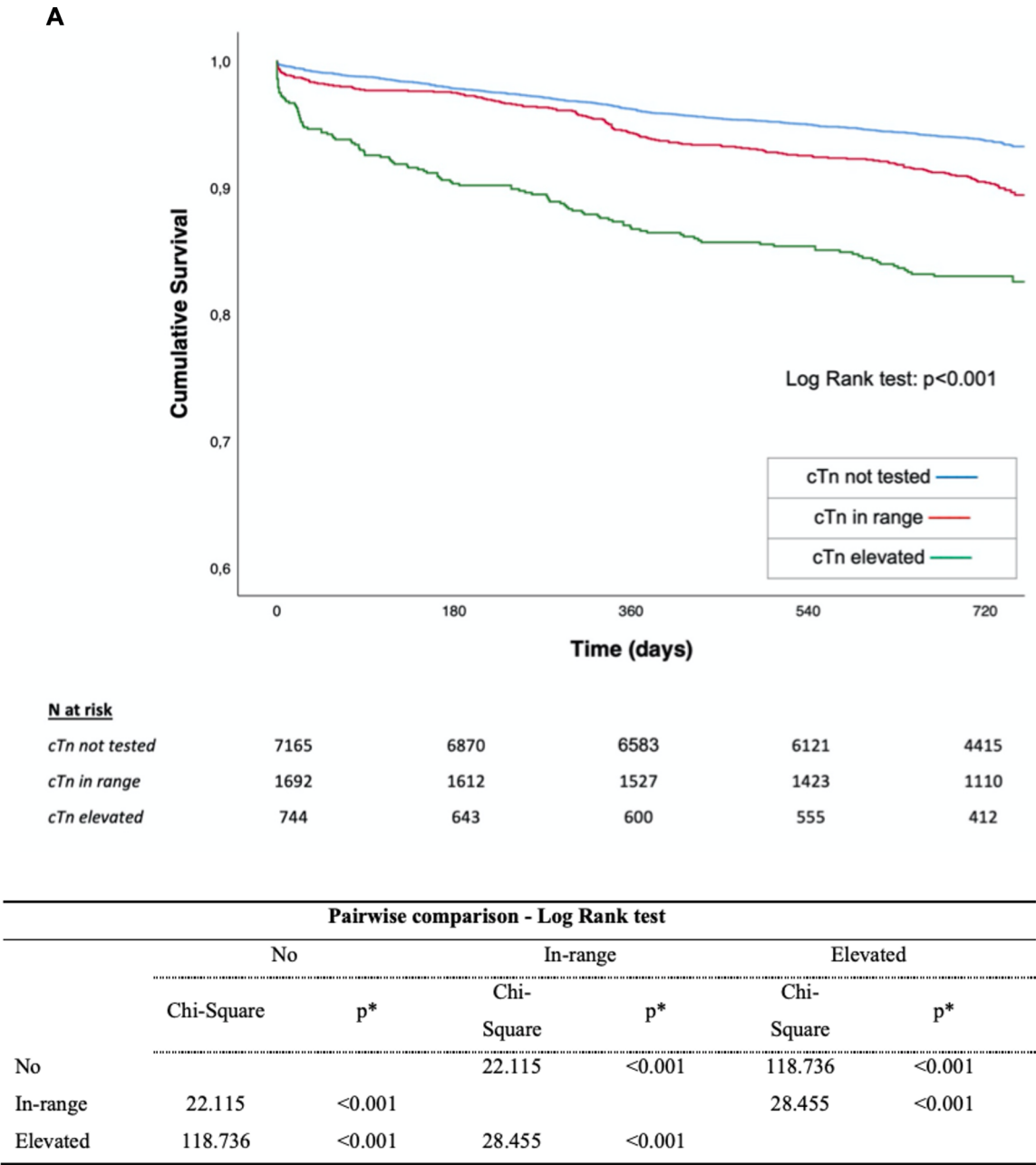
Fig. 1. Kaplan–Meier curves for main study outcomes according to cTn assessment Panel A. MACE (Any TE/ACS/CV death); Panel B. All-cause death Legend: ACS= acute coronary syndrome; cTn= cardiac troponins; CV= cardiovascular; MACE= major adverse cardiovascular events; TE= thromboembolic events. *= statistical significance is accepted at the p < 0.0167 level with Bonferroni correction.
