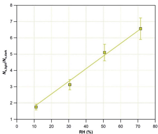
Fig. 6 The amplification factor, N_{S, \text{light}}/N_{S, \text{dark}} , plotted as a function of RH for Mýrdalssandur v-dust exposed to 75 ppb of SO 2 at T = 296 \text{ K} . The yellow line is the linear fit of the results.
