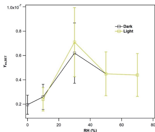
Fig. 7 Steady-state BET uptake coefficient, \gamma_{\text{SS,BET}} , as a function of RH during exposure of Mýrdalssandur v-dust to 75\text{ ppb} of \text{SO}_2 in the dark (black squares) and in the presence of UV light ( J_{\text{NO}_2} = 4.5 \times 10^{-3}\text{ s}^{-1} , yellow squares) at T = 296\text{ K} . Datapoints in the dark at 50% and 70% RH overlap with those under light.
