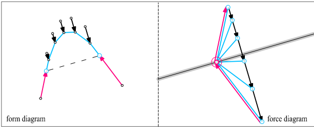
Figure 11. Application of a funicular structure.
