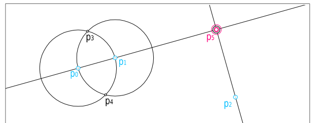
Figure 3. Detailed construction of a OrthoProj[p_0p_1p_2] constraint and application of this constraint to p_5 .
