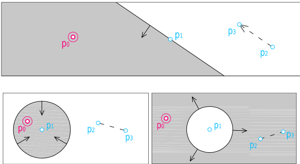
Figure 2. (up) a point p_0 that belongs to a HalfPlane[p_1p_2p_3] constraint; (bottom left) a point p_0 that belongs to a DiscInside[p_1p_2p_3] constraint; (bottom right) a point p_0 that belongs to a DiscOutside[p_1p_2p_3] constraint.
