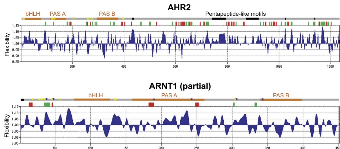
Fig. 4. Local flexibility analysis for Coryphaenoides armatus AHR and ARNT. Local flexibility values and associated graphs for both AHR2 (A) and ARNT1 (B) were predicted through the protein analysis toolbox of MacVector software. Above each plot is a scheme of the linearized primary structure (grey lines) with regions corresponding to basic helix-loop-helix (bHLH) and Per-Arnt-Sim (PAS) domains highlighted in orange. Also shown are positionally unique residue substitutions (yellow asterisks), including the most promising ones in the case of ARNT (blue asterisks), and regions that are only found in C. armatus proteins and not Microgadus tomcod homologs (black line; AHR, accession: ACI25083.1; ARNT, accession: ACX53265.1). Red and green vertical bars respectively reflect regions with increased or reduced local flexibility in C. armatus when compared to M. tomcod homologs.
