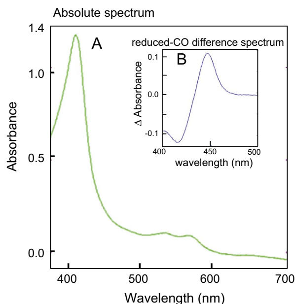
Fig. 6. Spectral Characterization of Coryphaenoides armatus CYP1A. C. armatus CYP1A was heterologously expressed in E. coli cells after N-terminal amino acid modification. A. The absolute oxidized spectrum was typical for a low-spin ferric cytochrome P450 enzyme. B. The reduced CO-difference spectrum Soret peak was located at about 450 nm, indicating a native P450 protein with a cysteine thiolate trans to the CO ligand to the heme iron.
