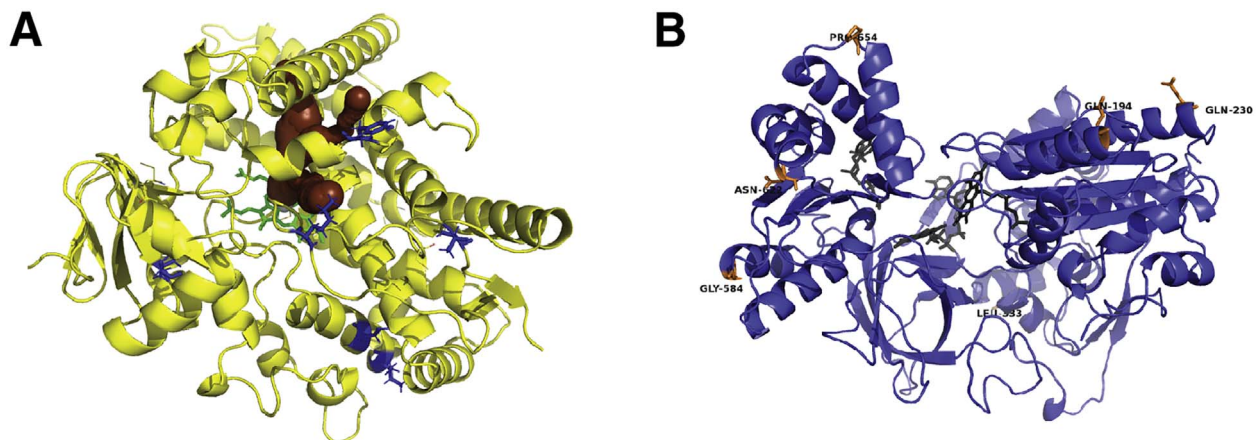
Fig. 1. Homology models of C. armatus CYP1A (A) and POR (B) showing location of residues unique to these deep-sea proteins. The models were generated using Modeller. The CYP1A structure was based on human crystal structures for CYP1A, and the access channels were calculated using Caver (see Material and methods ). The POR model was based on both human and rat POR crystal structures (see Material and methods ). The CYP1A model shows unique amino acids in blue, the locations of several calculated substrate access channels, in red, and the heme in green. Note that most of the unique residues are on the surface of the CYP1A, and that two are immediately adjacent to the largest substrate access channels. The POR model shows that most of the unique residues in POR also are on the surface of the protein (residues in orange; residue labeling is C. armatus residue number). The POR cofactors extracted from crystal structures are shown in black.
