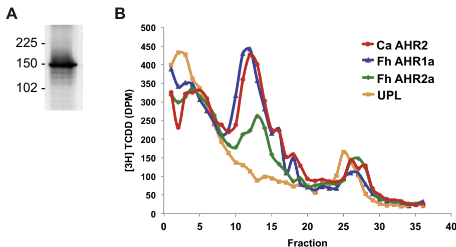
Fig. 5. Ligand binding assay with Coryphaenoides armatus AHR2. Ligand ( [^3\text{H}]\text{TCDD} ) specific binding to C. armatus (Ca) AHR2 along with AHR1a and AHR2a from F. heteroclitus (Fh) was assessed using sucrose density gradient centrifugation as described in Material and methods . A. Confirmation of in vitro expression of C. armatus AHR2 by incorporation of [^{35}\text{S}]\text{methionine} . Numbers indicate sizes of molecular weight markers. B. Binding of 2 nM [^3\text{H}]\text{TCDD} to the in vitro-expressed AHR proteins. Peaks of specific binding appear in fractions 10–15. Nonspecific binding was determined using reactions containing an empty vector (unprogrammed lysate, UPL).
