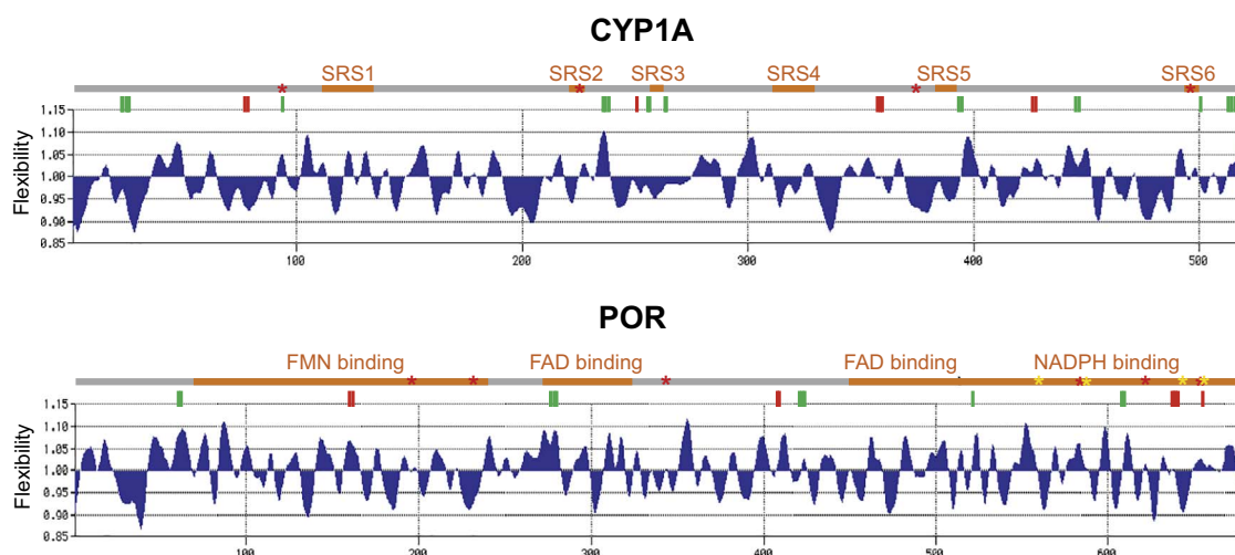
Fig. 2. Local flexibility analysis for Coryphaenoides armatus CYP1A and POR. Local flexibility values and associated graphs for both CYP1A (A) and POR (B) were predicted through the protein analysis toolbox of MacVector software. Above each plot is a scheme of the linearized primary structure (grey lines) with orange regions corresponding to substrate recognition sites (SRS) for CYP1A, and flavin mononucleotide (FMN), flavin adenine dinucleotide (FAD) and nicotinamide adenine dinucleotide phosphate (NADPH) binding regions for POR. Also shown are positionally unique residue substitutions (within vertebrates: red asterisks, within fish: yellow asterisks). Red and green vertical bars respectively reflect regions with increased or reduced basal flexibility in C. armatus when compared to the surface cod Gadus morhua (CYP1A, accession: ENSGMOP00000000312; POR, accession: ENSGMOP00000018048).
