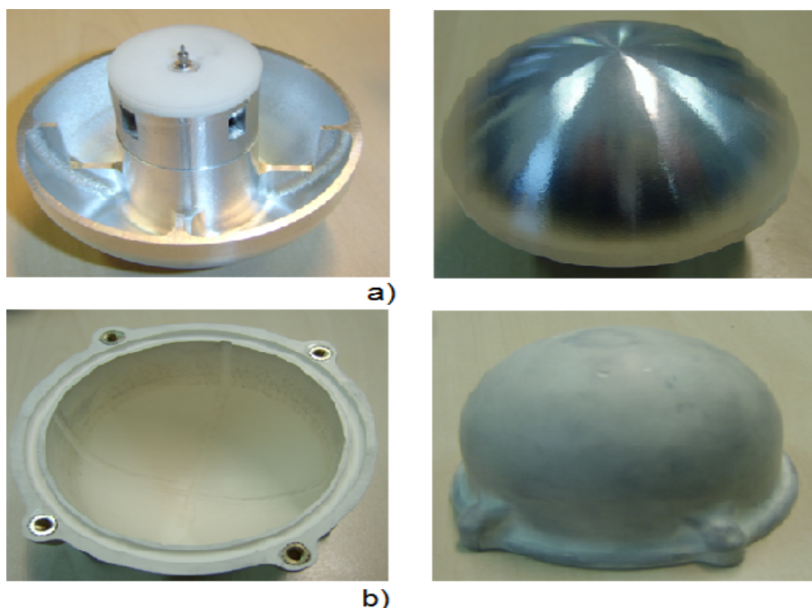
Figure 8.3: : a) The antenna body b) The protection layer.
