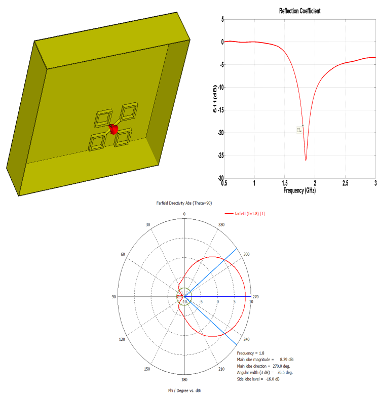
Figure 9.1: The GSM antenna geometry, the reflection coefficient and Radiation pattern at 1800 MHz, respectively.
