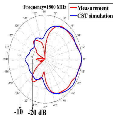
Figure 9.7: Comparison of the radiation patterns between the CST simulation and measurement for short-circuits auxiliary radiators
