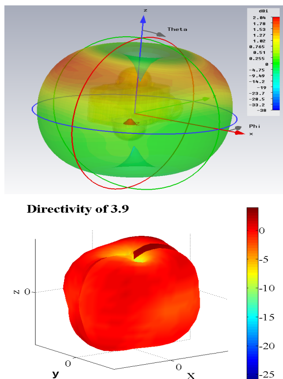
Figure 8.5: 3D radiation patterns from CST simulation and measurement at 868 MHz.
