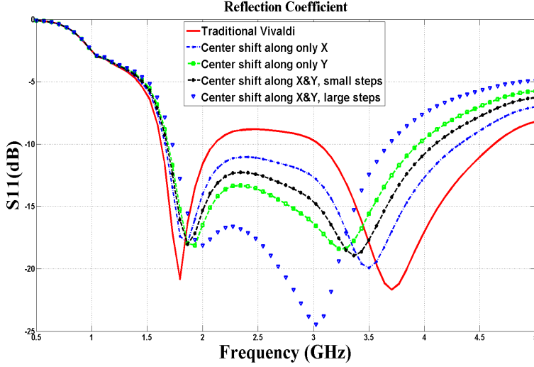
Figure 2.12: Reflection coefficients obtained by changing the ellipse center along X and Y axes.
