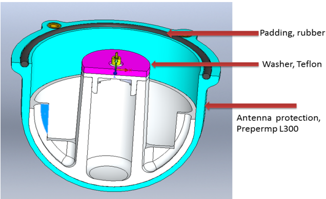
Figure 8.2: Bulb antenna components.
