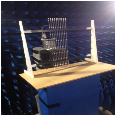
Figure 9.6: GSM antenna with short-circuits auxiliary radiators setup
