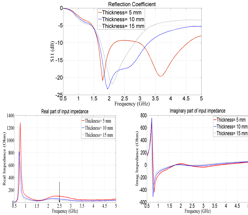
Figure 2.6: Effect of thickness on antenna impedance
