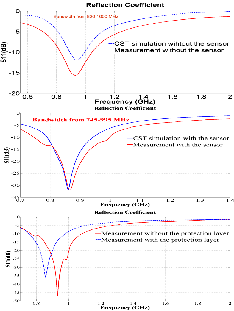
Figure 8.4: The reflection coefficient of the antenna with the sensor, without the sensor and the effect of the protection layer.
