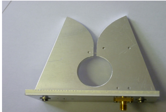
Figure 5.10: The 3D Vivaldi antenna prototype.
