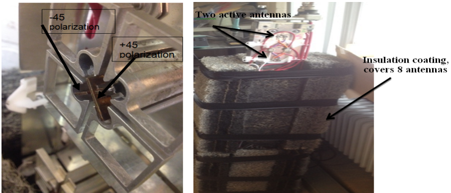
Figure 9.3: Kathrein sector antenna with insulation coating
