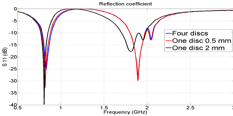
Figure 8.8: The influence of discs on the antenna bandwidth.
