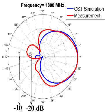
Figure 9.5: Comparison of the radiation patterns between CST simulation and measurement for free-space case at 1800 MHz
