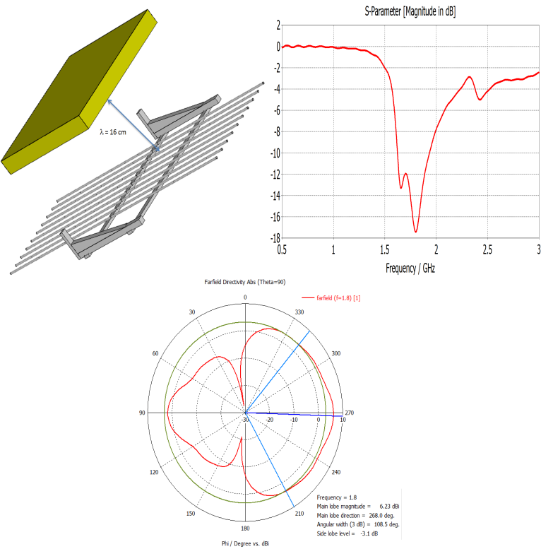
Figure 9.2: The effect of adding the auxiliary radiators
