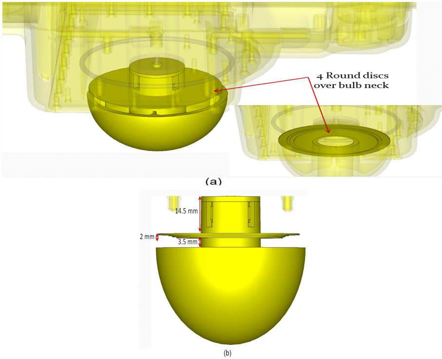
Figure 8.6: (a) The sensor with the dual-band antenna (b) four discs dimensions and positions.
