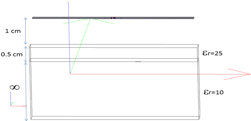
Figure 5.6: Horizontal dipole in the presence of a lossless multi-layered infinite ground; plot generated with IE3D.
