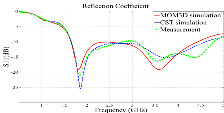
Figure 2.14: Comparison between reflection coefficients obtained from simulations MoM3D, and CST and measurement.
