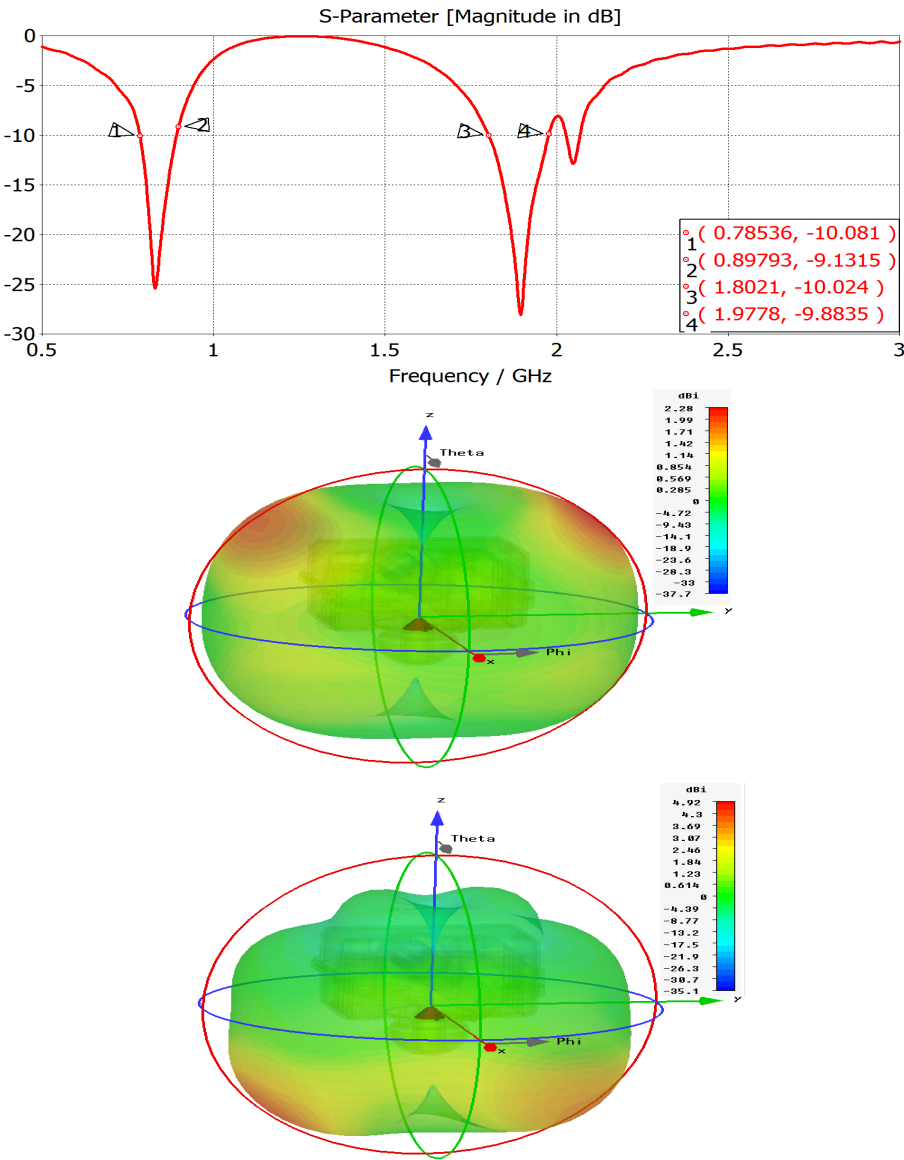
Figure 8.7: The reflection coefficient of the dual-band antenna with the radiation patterns at 900 and 1800 MHz, respectively.
