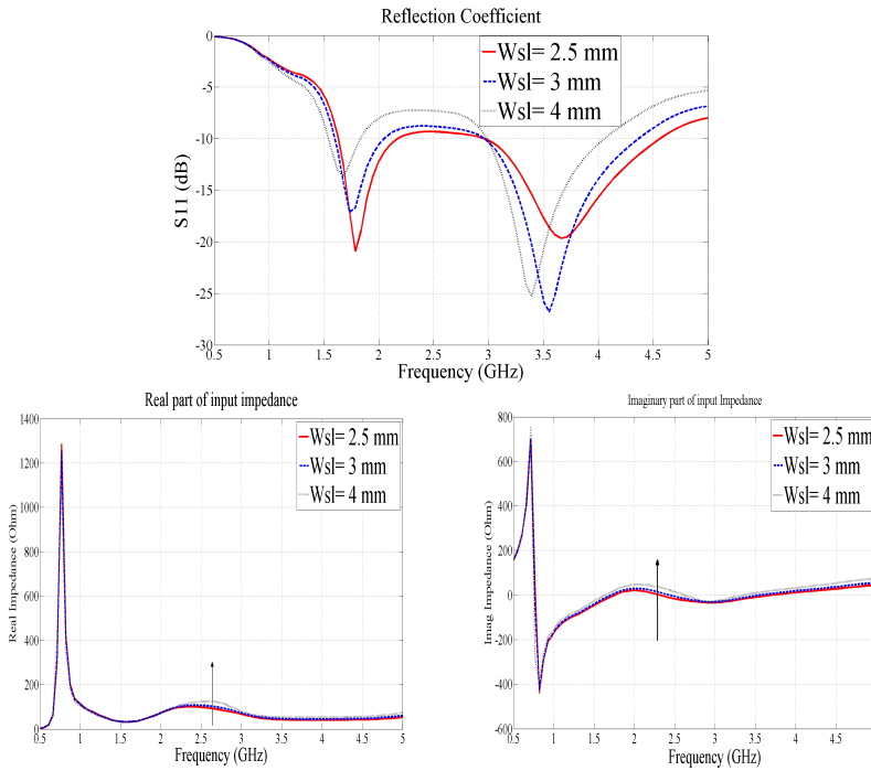
Figure 2.8: Effect of feed width on antenna impedance
