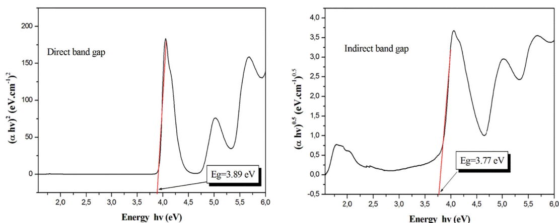
Fig. 14. Tauc Plots of (\alpha h\nu)^2 and (\alpha h\nu)^{0.5} versus the photon energy ( h\nu ).
