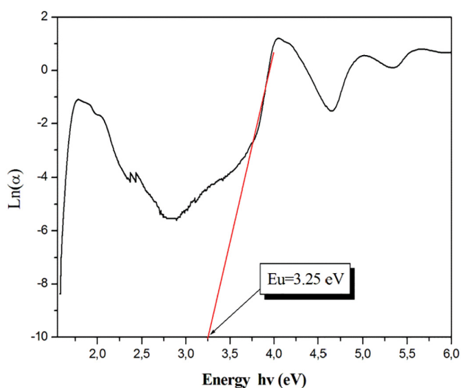
Fig. 15. \text{Ln}(\alpha) versus h\nu (photon energy) of the title compound.
