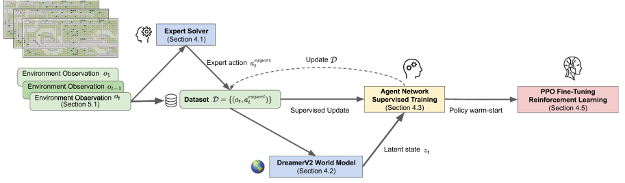
Fig. 1. Overview of our approach: (1) pretraining DreamerV2 world model, (2) collecting expert-labeled trajectories, (3) iterative supervised pretraining, and (4) fine-tuning with RL. Each main step is detailed in a specific subsection.
