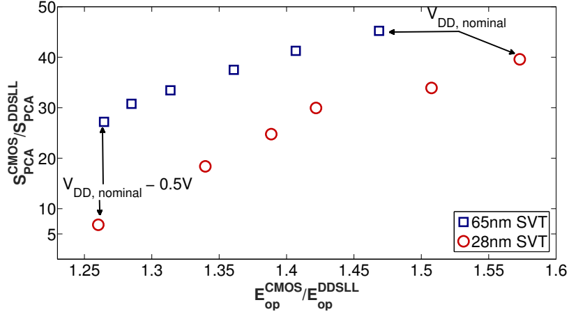
Fig. 2: Evolution of the tradeoff between the PCA signal ratio and the E_{op} ratio for CMOS vs. DDSLL using 65 & 28 nanometer technology nodes.
