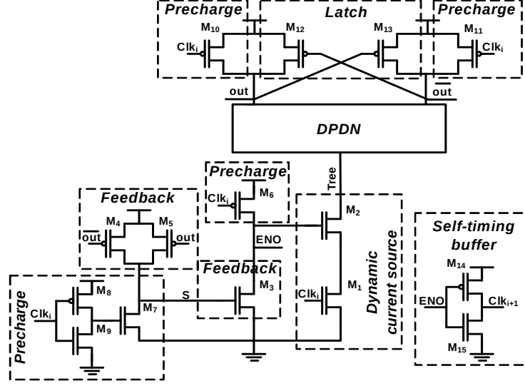
Fig. 1: Schematic of a generic DDSLL gate.
