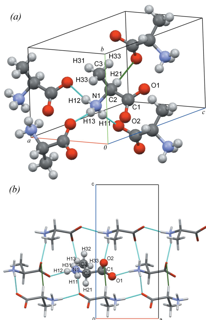
Figure 3 N—H \cdots O hydrogen bonds (blue dashed lines) and short C—H \cdots O contacts (green dashed lines) in L-alanine at 0.2 GPa. (a) This orientation illustrates that the different relative compressibility values of the three types of N—H \cdots O hydrogen bonds are closely interrelated with the orientation of the NH 3 + tail and its torsion motions. (b) Head-to-tail chains of zwitterions and the difference in types of N—H \cdots O hydrogen bonds formed by the two different O atoms are seen more clearly in this orientation. The numbering of atoms is shown. This figure is in colour in the electronic version of this paper.
