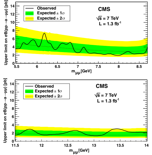
FIG. 2 (color online). Upper limits at 95% C.L. on \sigma \times \mathcal{B}(pp \rightarrow a \rightarrow \mu^+ \mu^-) in mass range 1 (upper panel) and mass range 2 (lower panel) including systematic uncertainties. The dotted lines correspond to the expected limits, and the bands correspond to 1- and 2- \sigma level uncertainties on the expected limits.
