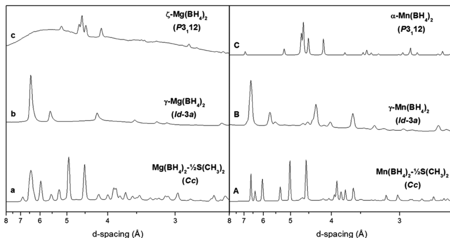
Fig. 2 Powder X-ray diffraction patterns for \text{Mg}(\text{BH}_4)_2 and \text{Mn}(\text{BH}_4)_2 polymorphs: (left) (a) \text{Mg}(\text{BH}_4)_2 \cdot 1/2\text{S}(\text{CH}_3)_2 , (b) \gamma\text{-Mg}(\text{BH}_4)_2 , (c) \zeta\text{-Mg}(\text{BH}_4)_2 shown in comparison to (right) (A) \text{Mn}(\text{BH}_4)_2 \cdot 1/2\text{S}(\text{CH}_3)_2 , (B) \gamma\text{-Mn}(\text{BH}_4)_2 and (C) \alpha\text{-Mn}(\text{BH}_4)_2 . Experimental details of X-ray data for the \text{Mg}(\text{BH}_4)_2 polymorphs presented here are found in the ESI.†
