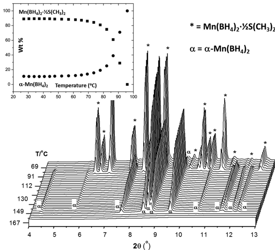
Fig. 4 In situ synchrotron radiation powder X-ray diffraction measured from room temperature to 200 °C of \text{Mn}(\text{BH}_4)_2 \cdot 1/2\text{S}(\text{CH}_3)_2 ( \lambda = 0.696713 Å, p(\text{Ar}) = 1 bar). Inset: Integrated intensities (wt%) of \text{Mn}(\text{BH}_4)_2 \cdot 1/2\text{S}(\text{CH}_3)_2 and \alpha\text{-Mn}(\text{BH}_4)_2 as a function of temperature. Filled circles: \alpha\text{-Mn}(\text{BH}_4)_2 , filled squares: \text{Mn}(\text{BH}_4)_2 \cdot 1/2\text{S}(\text{CH}_3)_2 .
