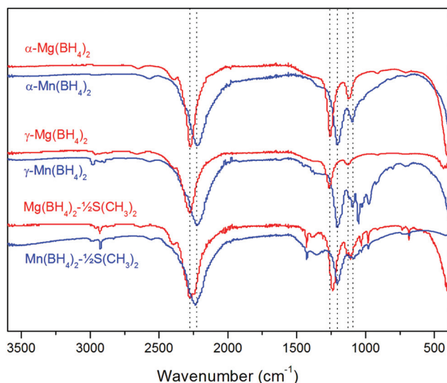
Fig. 3 Infrared spectroscopy for manganese and magnesium borohydride polymorphs. Red: \alpha\text{-Mg}(\text{BH}_4)_2 (top), \gamma\text{-Mg}(\text{BH}_4)_2 (middle), \text{Mg}(\text{BH}_4)_2 \cdot 1/2\text{S}(\text{CH}_3)_2 (bottom). Blue: \alpha\text{-Mn}(\text{BH}_4)_2 (top), \gamma\text{-Mn}(\text{BH}_4)_2 (middle), \text{Mn}(\text{BH}_4)_2 \cdot 1/2\text{S}(\text{CH}_3)_2 (bottom). Dotted lines to guide the eye.
