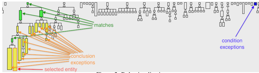
Figure 2: Rule visualization.
