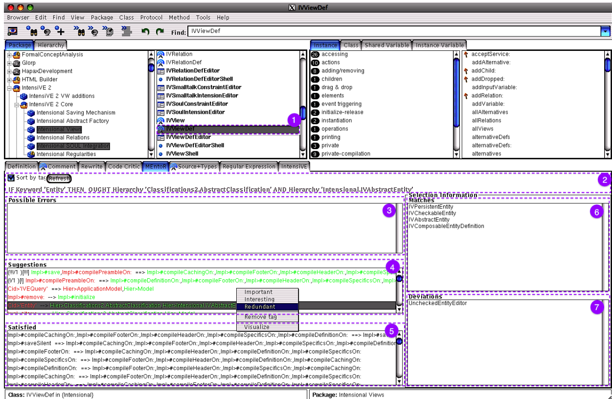
Figure 1: MEntoR's layout
