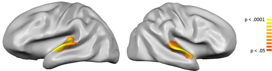
Figure 1: Whole brain activation map for listening to speech sounds versus silence across all subjects. The activation maps are projected on the inflated surface of the left and right hemispheres of one representative child. Maps are cluster size corrected (threshold = 20 voxels) at p < .05 .
