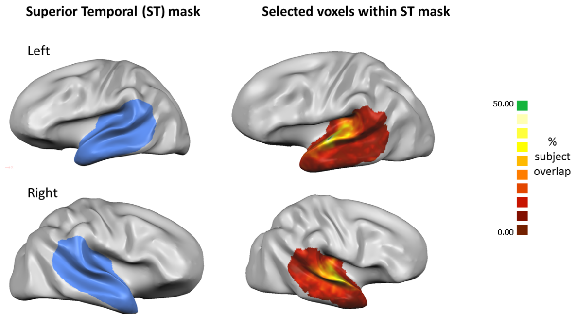
Figure 2: (a) Left and right Superior Temporal (ST) masks. The temporal masks are projected on the inflated surface of the left and right hemispheres of one representative child. (b) Probabilistic maps illustrating amount of subject overlap for the individually determined 500 most active voxels across the left and right temporal masks. The lighter the colour, the higher the across-subject consistency.
