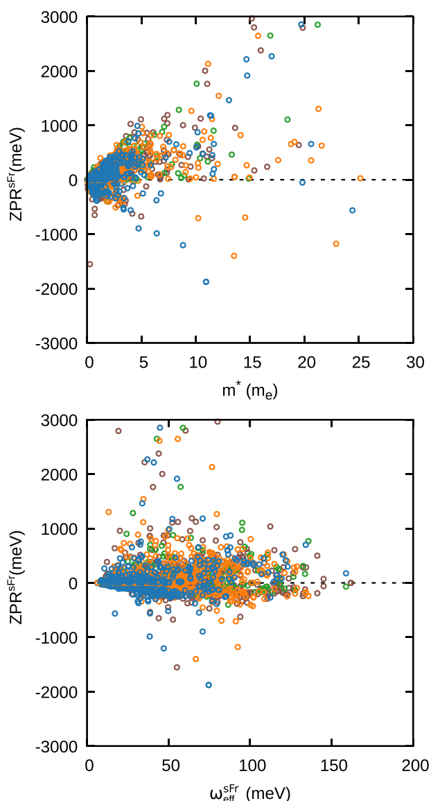
Fig. 2 Dispersion of conduction (negative) and valence (positive) ZPR sFr energies versus the effective mass, m_{\text{sFr}}^* (top), and effective phonon frequency, \omega_{\text{eff}}^{\text{sFr}} (bottom) for all materials with ZPR sFr below 3000 meV. Same conventions as in Fig. 1. A rough square root behavior (Equation (10)) governs the maximum accessible ZPR sFr for a given mass, and a degree of clustering is visible of the frequencies as a function of chemical period, with the lowest frequencies for halides, followed by chalcogenides, then the remaining materials. Dependence with the band effective mass (Eq. (32)) shows a dominant linear behavior, with a wider dispersion for valence bands when compared to the conduction band masses.
