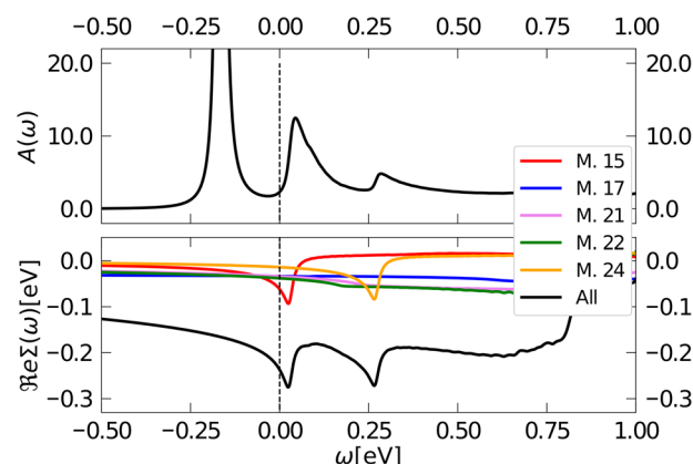
Fig. 7 Spectral function, A(\omega) (top) and the real part of the self-energy, \Re\Sigma(\omega) (bottom) for \text{KN}_3 at the CBM. The self-energy is split by phonon mode for the largest contributions to the \text{ZPR}_c as in Supplementary Table III. Only phonon modes 15 and 24 are LO, the others are non-LO.
