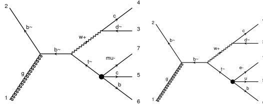
(c) One of the possible baryon number violating single top diagram, produced in association with a W boson.
