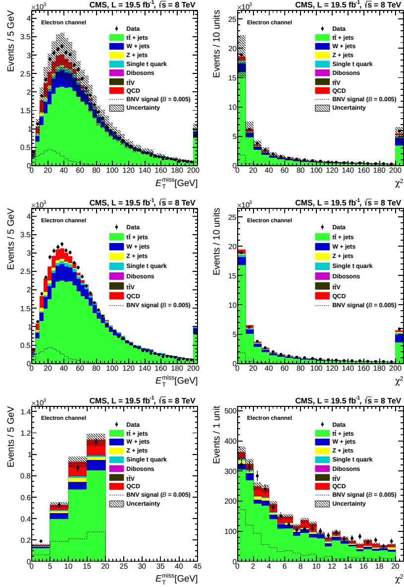
Figure 5.6: Electron analysis: distribution of E_T^{miss} (left) and \chi^2 (right) for basic (top), basic corrected (middle) and tight selection (bottom). The signal contribution expected for BR = 0.005 is also shown.
