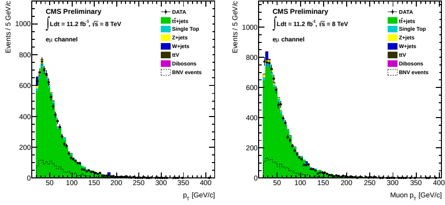
Figure 6.7: Dileptonic cross check: p_T distribution of the isolated muon and the isolated electron under the null hypothesis. Signal has been overlaid, assuming a branching ratio of 0.003.
