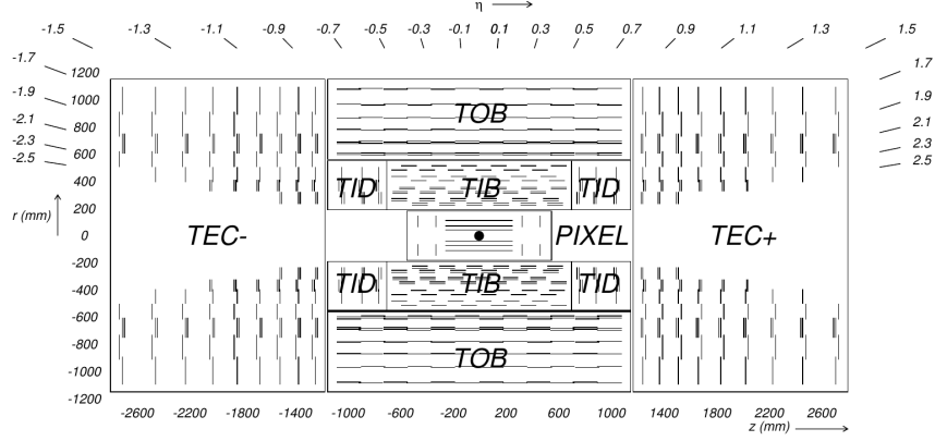
Figure 2.5: Schematic layout of CMS tracker; lines represent detector modules. The components are: Pixel Detector (PIXEL), Tracker Inner barrel (TIB), Tracker Outer barrel (TOB), Tracker Inner Disk (TID), Tracker endcap (TEC). [56]
