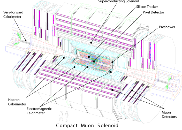
Figure 2.4: Schematic layout of Compact Muon Solenoid detector [56].
