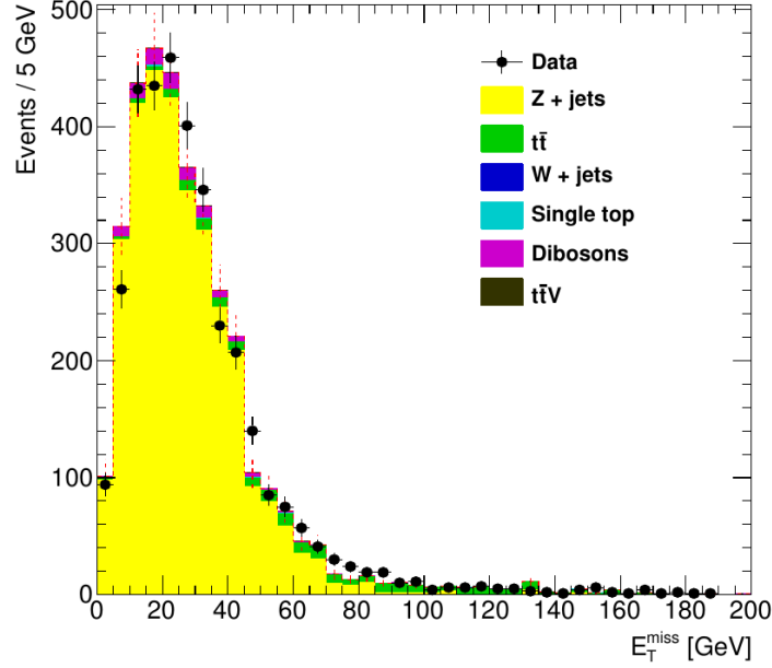
Figure 6.5: 2012 Analysis: distributions of E_T^{\text{miss}} miss in both data and simulation for a sample events enriched of Z+4 \text{ jets} \rightarrow \mu^+\mu^- + 4 \text{ jets} events. For both data and simulation the error bars indicate the statistical uncertainty.
