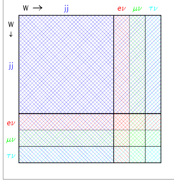
Figure 1.3: Top quark decay modes are shown, where: BR(t\bar{t} \rightarrow b\bar{b}q\bar{q}'\bar{q}') = 44\% , BR(t\bar{t} \rightarrow b\bar{b}q\bar{q}'l\nu_l) = 30\% and BR(t\bar{t} \rightarrow b\bar{b}l'l\nu_l) = 5\% . [12]
