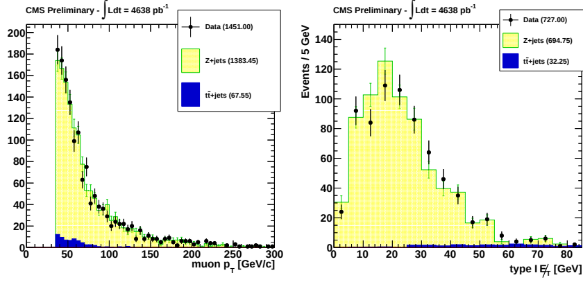
Figure 6.4: 2011 Analysis: distributions of muon p_T (left) and E_T^{miss} miss (right) in both data and simulation for a sample events enriched of Z+4 \text{ jets} \rightarrow \mu^+ \mu^- + 4 \text{ jets} events. For both data and simulation the error bars indicate the statistical uncertainty.
