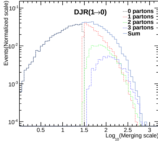
Figure 3.1: Differential Jet Ratio for a t\bar{t} + 1,2,3,4 jets sample at 8 TeV. This plot represents the distribution of the transition value Q , namely the value of the resolution for which an n jet event becomes an n - 1 jet event (in this case, the transition from 1 to 0 jets is shown). The plot has been produced using Pythia6 on top of a MG5 sample, setting q_{cut} to 30 GeV. The contribution of one, two three and four extra parton events are shown, as well as the total number of events (in light blue).
