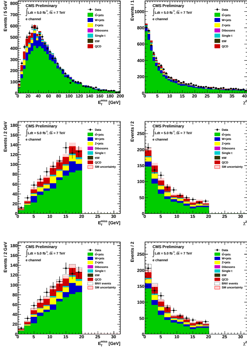
Figure 5.3: Electron analysis: distribution of E_T^{\text{miss}} (left) and \chi^2 (right). Top: corrected basic selection with a null assumed BR value. Middle: tight selection with a null assumed BR value. Bottom: tight selection with an assumed BR value equal to 0.003.
