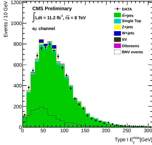
Figure 6.8: Dileptonic cross check: E_T^{\text{miss}} distribution of simulated and observed transverse missing energy in the null hypothesis. Signal has been overlaid, assuming a branching ratio of 0.003. An excess of 6.4% can be observed in the first two bins. Yet the contribution of BNV signal in the low energy bins is not negligible and does not allow to draw a definitive conclusion about the agreement between simulated and observed E_T^{\text{miss}} for very low missing energy values.
