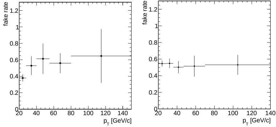
Figure 4.6: 2012 analysis: Fake rate F as function of p_T for muon (left) and electron channel (right). Error bars are statistical uncertainty only.
