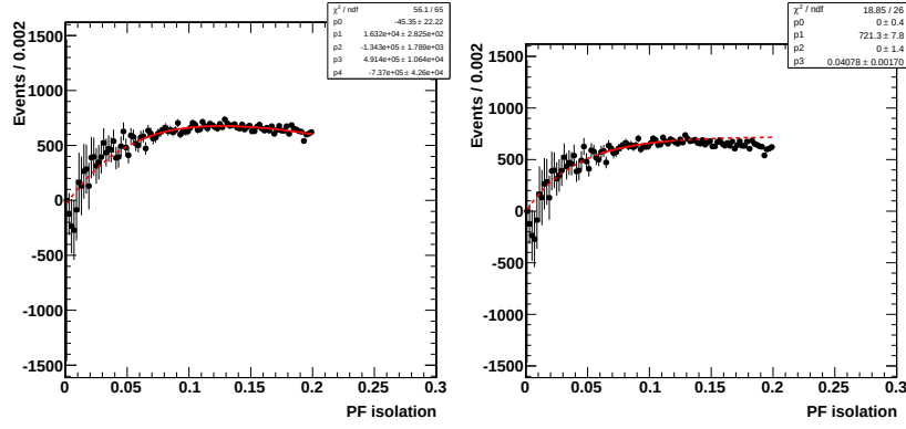
Figure 4.10: 2011 electron analysis: fourth degree polynomial (left) and exponential (right) fit of the difference between I_{\text{Rel}}^{\ell} in data and MC (only for non-QCD processes) for events with an electron and at least 3 jets with p_T > 30 GeV/c.
