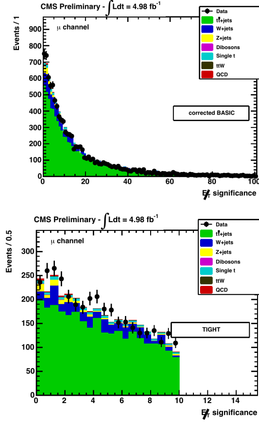
Figure 6.1: Muon analysis: E_T^{\text{miss}} significance distributions for the corrected BASIC (top) and TIGHT (bottom) selections under the assumption null BR, using the E_T^{\text{miss}} significance algorithm with cut value at 10.
