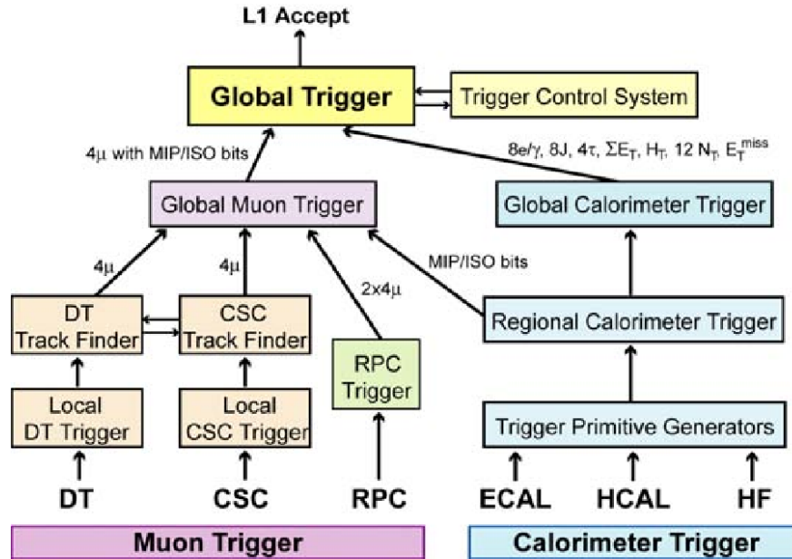
Figure 2.14: Architecture of Level-1 Trigger [56].
