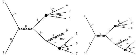
(b) One of the possible baryon number violating diagrams for t\bar{t} pairs in muon and electron channel, where both the top quarks undergo BNV decay.
