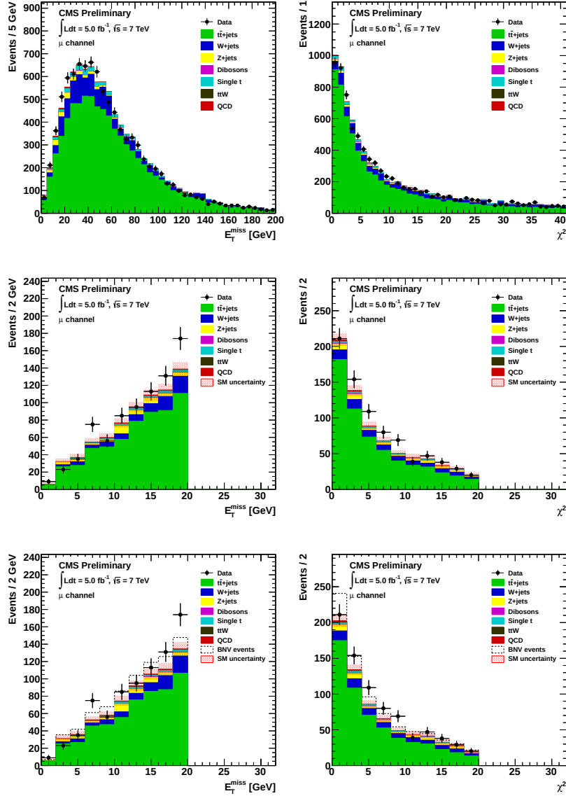
Figure 5.2: Muon analysis: distribution of E_T^{\text{miss}} (left) and \chi^2 (right). Top: corrected basic selection with a null assumed BR value. Middle: tight selection with a null assumed BR value. Bottom: tight selection with an assumed BR value equal to 0.003.
