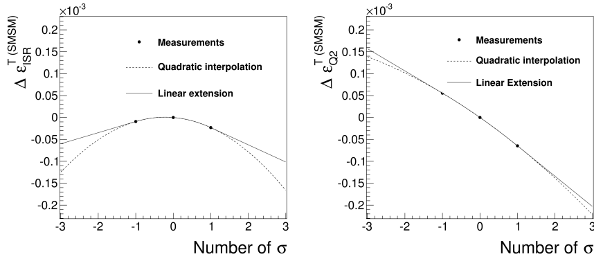
Figure 5.1: Absolute impact of initial/final state radiation (left) and factorization scales (right) on \epsilon_{H,SM\_SM}^T as function of the shift from the central value, expressed as number of sigmas. Each uncertainty source has been fluctuated of plus (minus) one sigma, then the efficiency to pass basic selection has been recalculated. The three points have been interpolated by a quadratic functional form ( y = ax^2 + bx + c ); a regularization has been made extending the interpolating function in a linear fashion outside [-1, 1] sigma interval.
