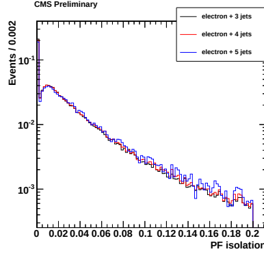
Figure 4.7: Distribution of I_{\text{Rel}}^{\ell} for a simulated t\bar{t} sample with at least 3,4,5 jets with p_T > 30 \text{ GeV}/c : changes in shape are almost negligible.
