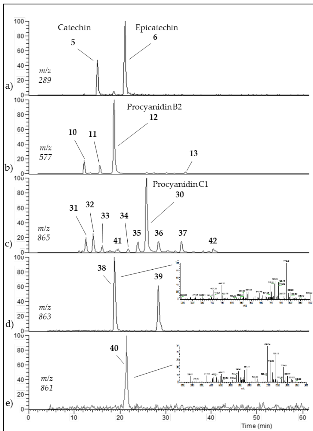
Figure 1. RP-HPLC-MS/MS(ESI(-)) chromatograms, recorded at (a) m/z=289 , (b) m/z=577 , (c) m/z=865 , (d) m/z=863 , and (e) m/z=861 , of procyanidin C1 model medium heated for 12 h at 90 °C. Corresponding structures in Table 1.
