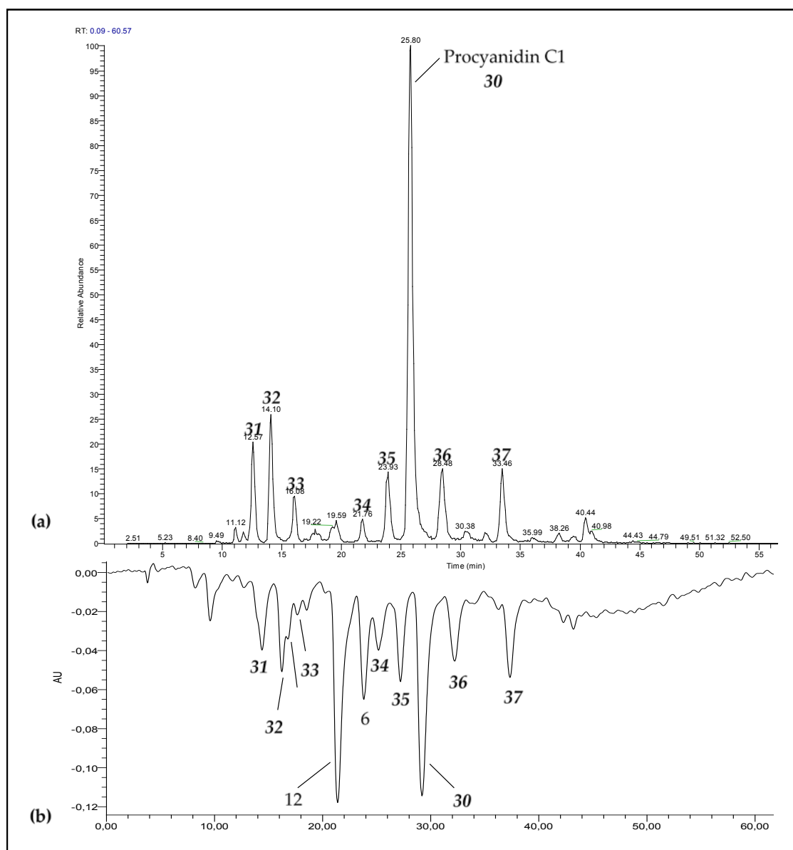
Figure 4. (a) RP-HPLC-MSMS(ESI(-)) chromatograms recorded at m/z=865 , 577 , and 289 . (b) RP-HPLC-online TEAC chromatogram after the reaction with ABTS^{+\bullet} ( 642\text{ nm} ) for procyanidin C1 model medium heated for 12\text{ h} at 90\text{ }^{\circ}\text{C} .
