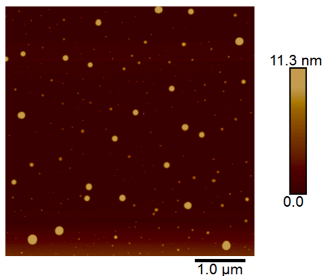
Fig. 2. - Atomic force microscopy images of SO-NC (scale 5 × 5 μm).
