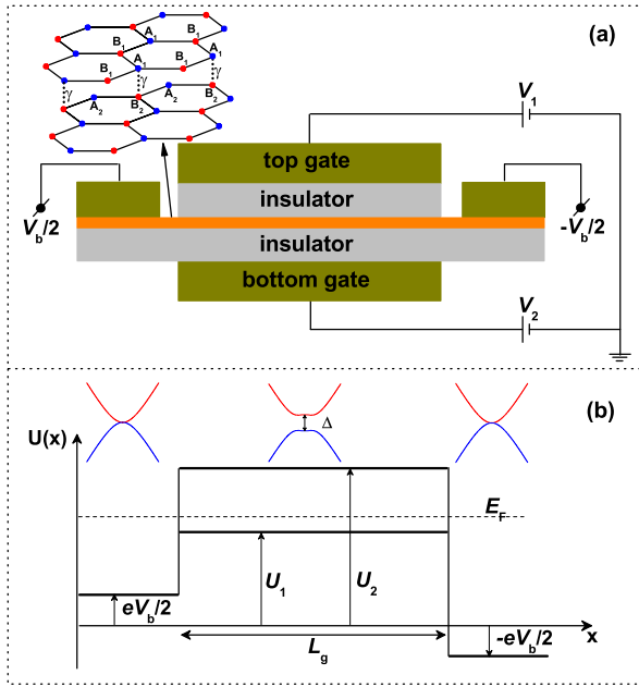
Figure 1. (a) Schema and (b) potential energy diagram of the considered structure.
