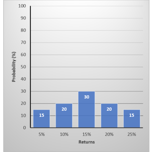
Figure 3: Distribution of the stock index fund returns
