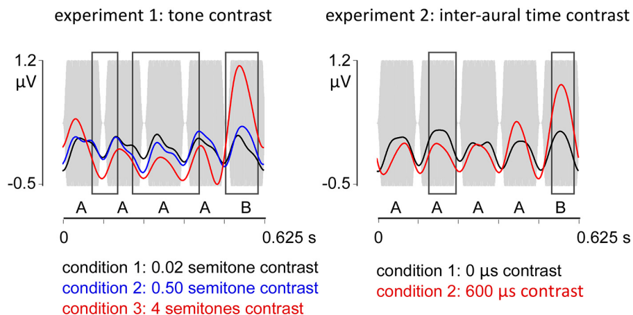
Fig. 5. Time course of the EEG responses to the AAAAB pattern. Gray bars represent the pattern envelope. In the 2 experiments, responses to each tone were observed as positive deflections peaking at \sim 50 ms, followed by a negative deflection at \sim 100 ms. A point-by-point comparison (cluster statistics) across conditions revealed significant differences across conditions during and also after the presentation of the B tone (black boxes), which are thus compatible with middle and late latency auditory potentials, respectively, triggered by the contrast.
