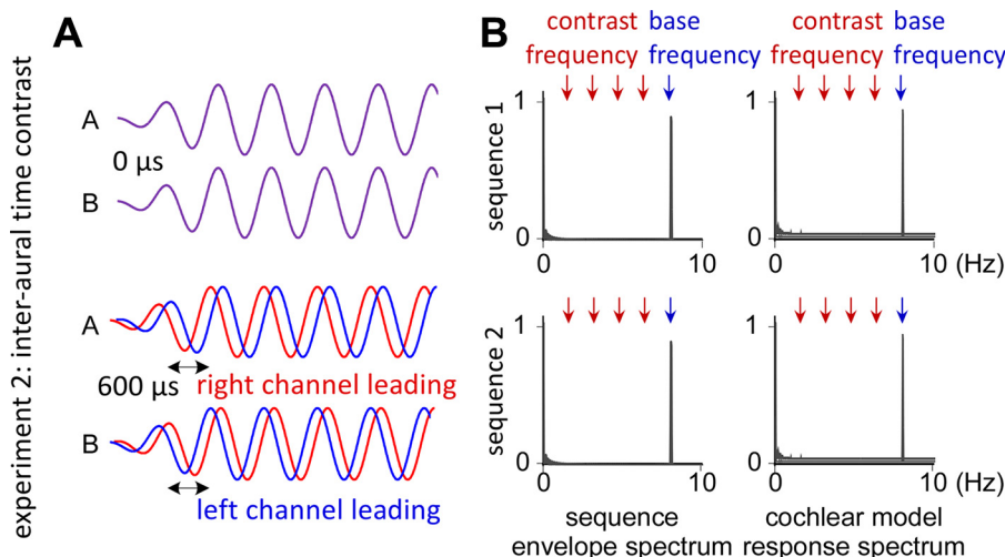
Fig. 2. Stimuli of experiment 2 with interaural time contrast. A: in condition 1 , there was no interaural time contrast between A and B tones (top). In condition 2 , the A and B tones were presented with an interaural time contrast of 600 \mu s (bottom), inducing an illusion of 180° azimuth contrast between A and B tones and thus an effect of stream segregation due to the perceived separate spatial sources. B: frequency spectrum of the sound envelope and of the cochlear signals obtained using a cochlear channel model of response (displayed as normalized relative to the maximum magnitude within each sequence). Note that, in both conditions, no peaks emerge at contrast frequencies, because interaural time contrasts cannot be processed by cochlear channels.
