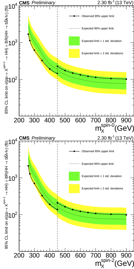
Figure 3.18: Expected and observed 95% CL s upper limits on the the resonant Higgs pair production cross section times branching fraction for hh \rightarrow bbVV \rightarrow bbl\nu\bar{\nu} , computed using the asymptotic CL s method. Spin-0 results are shown on the top plot and spin-2 limits are visible on the bottom plot. The markers correspond to limits evaluated on fully-simulated signal samples, while in between fully-simulated samples the limits have been set on interpolated signal yields and systematics.
