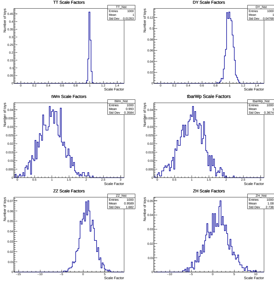
Figure 4.9: Scale factors for the six SM processes obtained from a maximum likelihood fit to pseudo-data. The distribution used to perform the fit is the yields in each of the final box resulting from the nominal splitting. A thousand pseudo-data experiments have been generated according to Poisson distribution with a mean corresponding to the expected yields considering the six SM processes.
