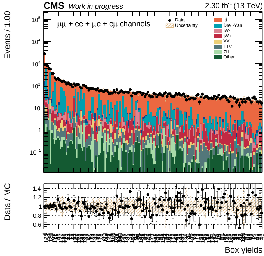
Figure 4.6: Yields in each of the final boxes resulting from the recursive phase space splitting with \epsilon_{\text{cut}} = 2 and \text{Stat}_{\text{cut}} = 0.1 . The histogram bins have been sorted by decreasing SM expected yield.
