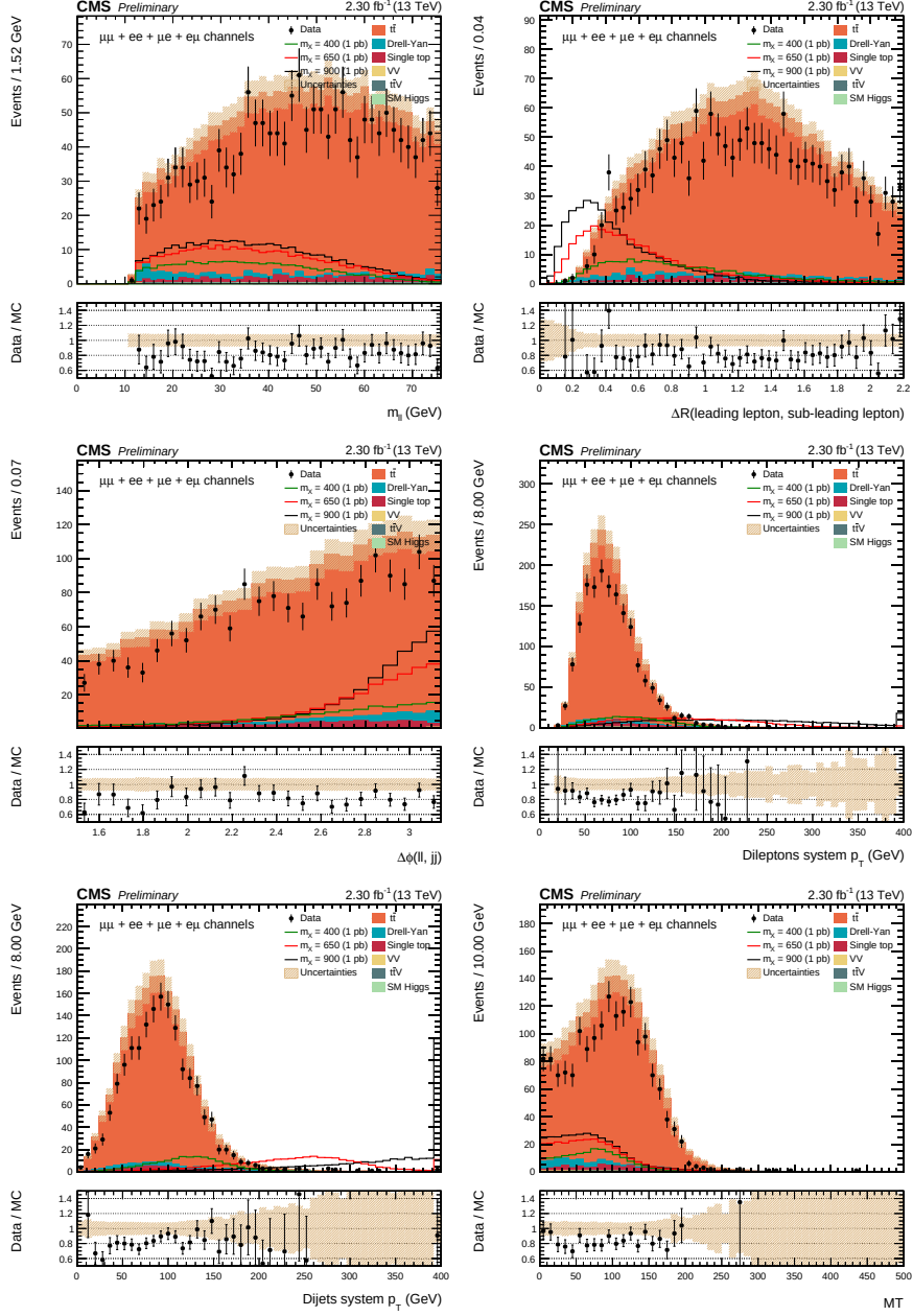
Figure 5.3: BDT training input variables that are not shown in the text body. From top left to bottom right: m_{\ell\ell} , \Delta R_{\ell\ell} , \Delta\phi_{\ell\ell, jj} , p_T^{\ell\ell} , p_T^{jj} , and MT distributions for data and simulated events after requiring all selection cuts described in Sec. 3.3. All lepton flavour combinations are shown together.
