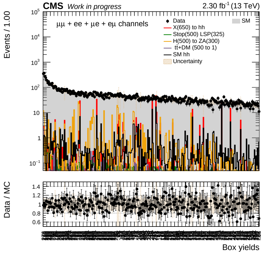
Figure 5.6: Yields in each of the final boxes resulting from the recursive phase space splitting with \epsilon_{\text{cut}} = 1.5 and \text{Stat}_{\text{cut}} = 0.1 . The histogram bins have been sorted by decreasing SM expected yield and the uncertainty band contains all the uncertainties described in Sec. 3.5 except for the normalization uncertainties. The histogram is shown with all the SM processes merged.
