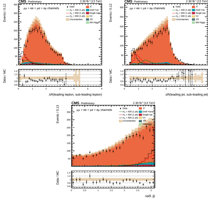
Figure 3.6: \Delta R_{\ell\ell} , \Delta R_{jj} , and \Delta\phi_{\ell\ell,jj} distributions for data and simulated events after requiring two leptons, two b-tagged jets, and m_Z - m_{\ell\ell} > 15 GeV. All lepton flavour combinations shown together.
