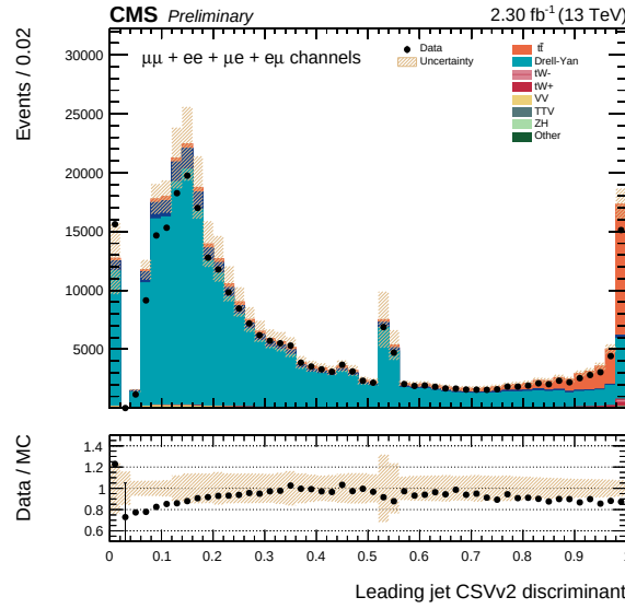
Figure 2.12: CSVv2 discriminant for the jet with highest CSVv2 in events containing at least two leptons and two jets. Jets without a selected track and secondary vertex are arbitrarily assigned a discriminator value of -10. The rightmost bin includes all events from the overflow, while the underflow is added to the first bin. No b-tagging MC correction is applied on this distribution.
