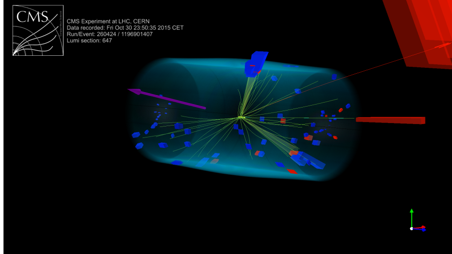
Figure 2.14: Display of a typical llbb event recorded by the CMS experiment during the 2015 data taking era. Tracks are represented by yellow lines, electromagnetic(hadronic) calorimeter deposit by red(blue) blocks and the missing transverse energy is shown as a purple arrow. The event shown belongs to the e\mu category and has been analyzed in this work.
