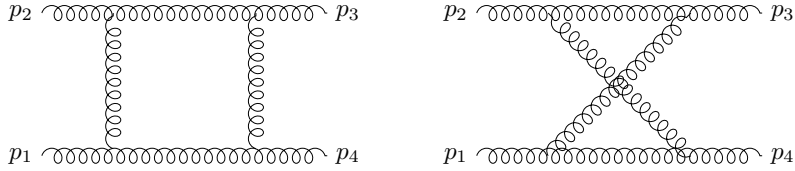
Figure 3.4: The dominant one-loop amplitudes in multi-Regge kinematics.
