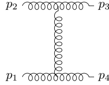
Figure 3.3: The dominant tree-level amplitude in multi-Regge kinematics.
