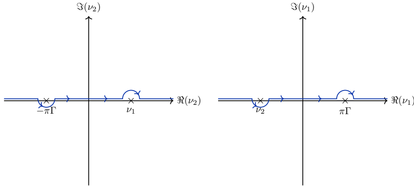
Figure 3.10: The integration contours for seven-particle scattering in MRK.
