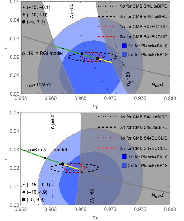
Figure 1: The diagonal line represents values of n_s and r predicted by the RGI model (upper panel) and \alpha -T model (lower panel) for fixed \alpha , with the inflaton coupling varying along the curve. The black discs indicate the predictions for specific values of a Yukawa coupling y , with (\log_{10} y, \log_{10} T_{\text{re}}/\text{GeV}) given in the legend. Conditions (3) and (4) are fulfilled in the green part, the gray parts are ruled out by the conditions N_{\text{re}} > 0 and T_{\text{re}} < T_{\text{BBN}} . Ellipses indicate current constraints and future sensitivities to n_s and r , N_k is the number of e -folds between the horizon crossing of a perturbation with wave number k and the end of inflation (12).
