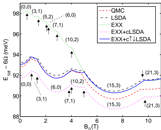
FIG. 1: (color online). Total ground-state energy (minus 6\Omega = 6\sqrt{\omega_0^2 + \omega_z^2}/4 ) in a six-electron quantum dot as a function of external magnetic field (SI units). The results have been calculated using the exact-exchange (EXX), EXX with LSDA correlation (EXX+cLSDA), and EXX with the corrected LSDA correlation (EXX+c \uparrow\downarrow LSDA). The LSDA and quantum Monte Carlo (QMC) results 8 are shown for comparison. The arrows mark the points where the ground-state configuration ( L_z, S_z ) changes.
