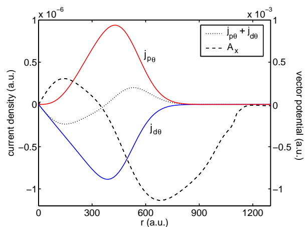
FIG. 2: (color online). Angular components of the paramagnetic and diamagnetic currents, j_{p\theta} and j_{d\theta} , and their sum for the (-21, 3) state at B_0 = 11 T. The dashed line shows the exchange vector potential for the same configuration.
