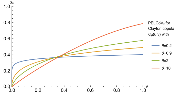
Fig. 4. Function v \mapsto u_v for the Clayton copula with different values of the dependence parameter.
