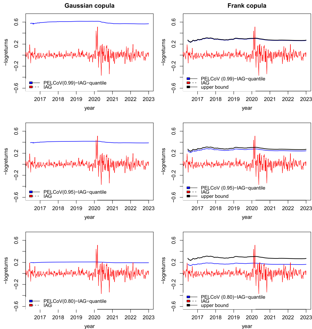
Fig. 15. Given the bivariate time series (X_t, Y_t) , the left-hand plots show the time series X_t (log-returns of IAG) together with their u_v -quantiles for v = 0.99, 0.95 and 0.80 , respectively, under the assumption of a time-varying Gaussian copula. The right-hand plots show the time series X_t , together with their u_v -quantiles for v = 0.99, 0.95 and 0.80 , respectively, and with their upper bounds (given by the u^* -quantiles) under the assumption of a time-varying Frank copula.
