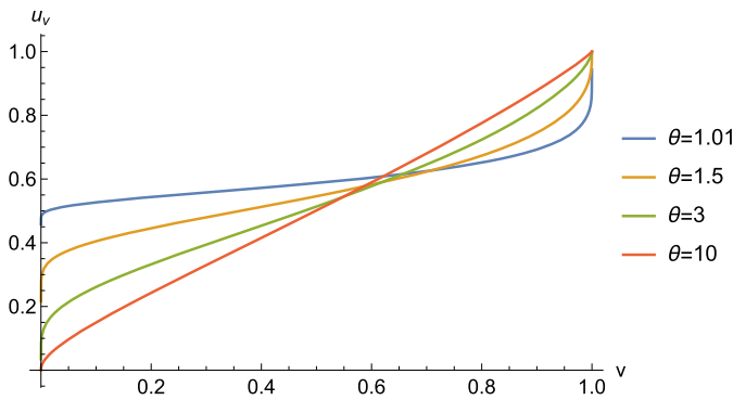
Fig. 10. Function v \mapsto u_v for the Gumbel Hougard copula with different values of the dependence parameter.
