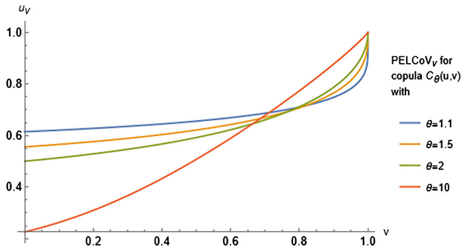
Fig. 11. Function v \mapsto u_v for the copula 4.1.6 in Nelsen (2007) with different values of the dependence parameter.
