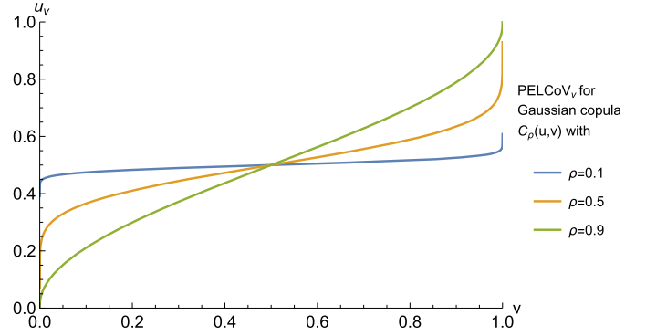
Fig. 9. Function v \mapsto u_v for the Gaussian copula with different values of the dependence parameter.
