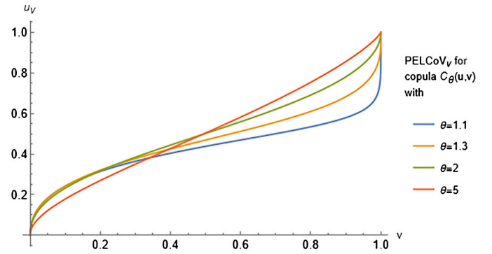
Fig. 13. Function v \mapsto u_v for the copula 4.1.14 in Nelsen (2007) with different values of the dependence parameter.
