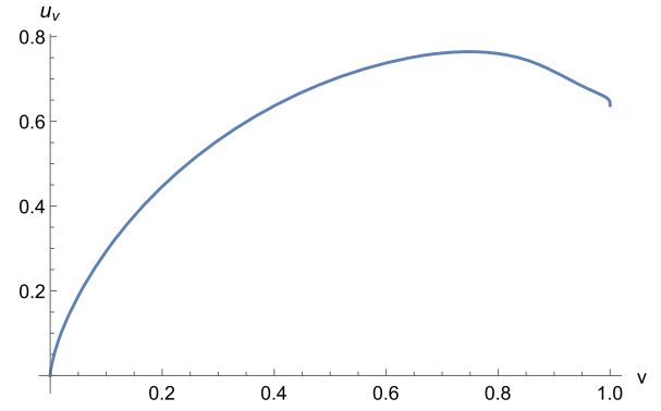
Fig. 2. Function v \mapsto u_v for the vector (X, Y) , where Y = X + W , where X \sim \text{Exp}(1) , W \sim \text{Weibull}(0.5, 1) and X and W are independent.
