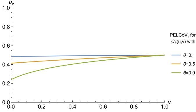
Fig. 5. Function v \mapsto u_v for the Ali-Mikhail-Haq copula with different values of the dependence parameter.
