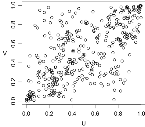
Fig. 14. Scatter-plot of the empirical copula of the bivariate time series (X_t, Y_t) , given by (F_t(x_t; \hat{\lambda}_1), G_t(y_t; \hat{\lambda}_2)) .
