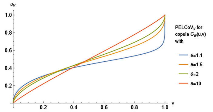
Fig. 12. Function v \mapsto u_v for the copula 4.1.12 in Nelsen (2007) with different values in the dependence parameter.
