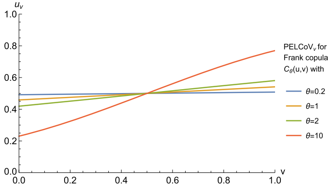
Fig. 3. Function v \mapsto u_v for the Frank copula with different values of the dependence parameter.
