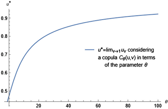
Fig. 7. Function \theta \mapsto u^* = \lim_{v \rightarrow 1} u_v for the copula (4.1.17) in Nelsen (2007).
