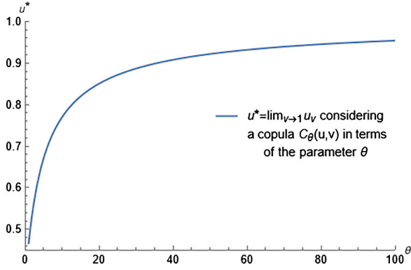
Fig. 6. Function \theta \mapsto u^* = \lim_{v \rightarrow 1} u_v for the copula (4.1.13) in Nelsen (2007).
