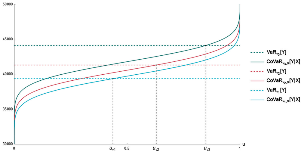
Fig. 1. PELCoV v values for v_1 = 0.4, v_2 = 0.7 and v_3 = 0.95 for a normal vector (X, Y) with \mu_X = 10000, \sigma_X = 1000, \mu_Y = 40000, \sigma_Y = 2500 and \rho = 0.9 . (For interpretation of the colours in the figure(s), the reader is referred to the web version of this article.)
