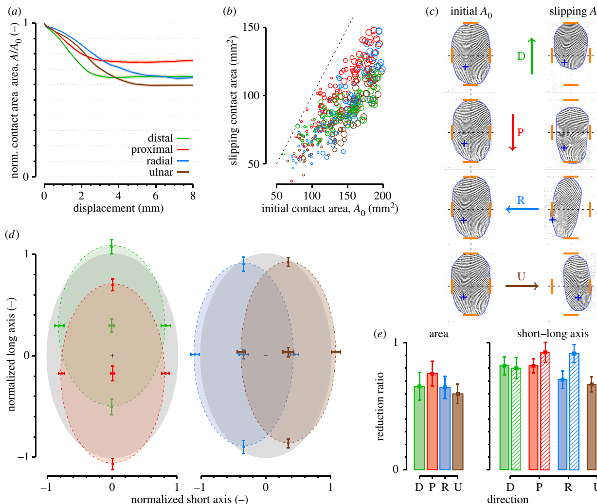
Figure 5. (a) Evolution of the contact area as a function of stimulus displacement. Solid lines are means among all trials. Shaded areas represent standard error. (b) Scatter plot of initial contact area versus slipping contact area during steady-state slipping. Circle sizes correspond to the three normal force conditions (0.5, 1 and 2 N). Direction of movement is represented by different colours. Dashed line represents equal contact areas (slope = 1). (c) Example images of the initial contact area (left) and slipping contact area (right) in each direction (D, P, R and U) from subject S3. Orange dashes report external limits (top, bottom, left and right) of the initial contact and a blue cross is attached to the papillary whorl. (d) Normalized shape of the contact region. Left: proximal and distal. Right: radial and ulnar. Grey ellipse represents normalized initial contact area. Coloured ellipses represent mean contact region during slipping. Central cross represents mean geometrical centre. Four corner points represent mean external borders of the contact area. Error bars represent standard deviation. (e) Reduction ratios between initial contact area and slipping contact area. Right panel: Shaded bars represent short axis, hatched bars represent long axis. Error bars represent the standard deviation.
