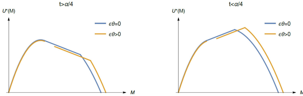
Fig. 6. Equilibrium utility as function of population size.
