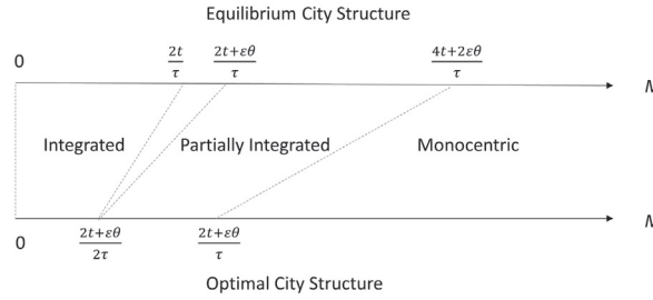
Fig. 7. Equilibrium &amp; optimal city structures.
