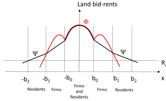
Fig. 3. Equilibrium land rents in partially integrated cities.
