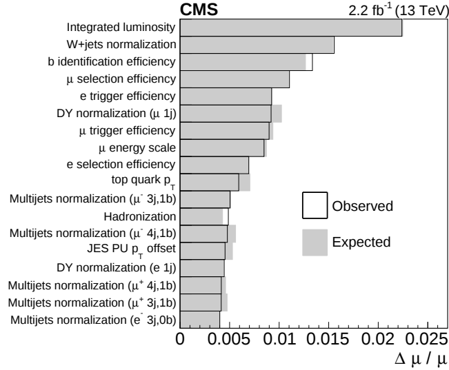
Figure 1.8: Estimated impact—change in the expected and observed signal strength—resulting from the listed sources of experimental and theoretical uncertainty in the \sigma_{t\bar{t}} analysis of Ref. [75]. The various contributions are shown from the largest to the smallest observed impact. The dominant source of uncertainty is related to the integrated luminosity, which is expected and observed to impact the signal strength at the level of 2.2%.
