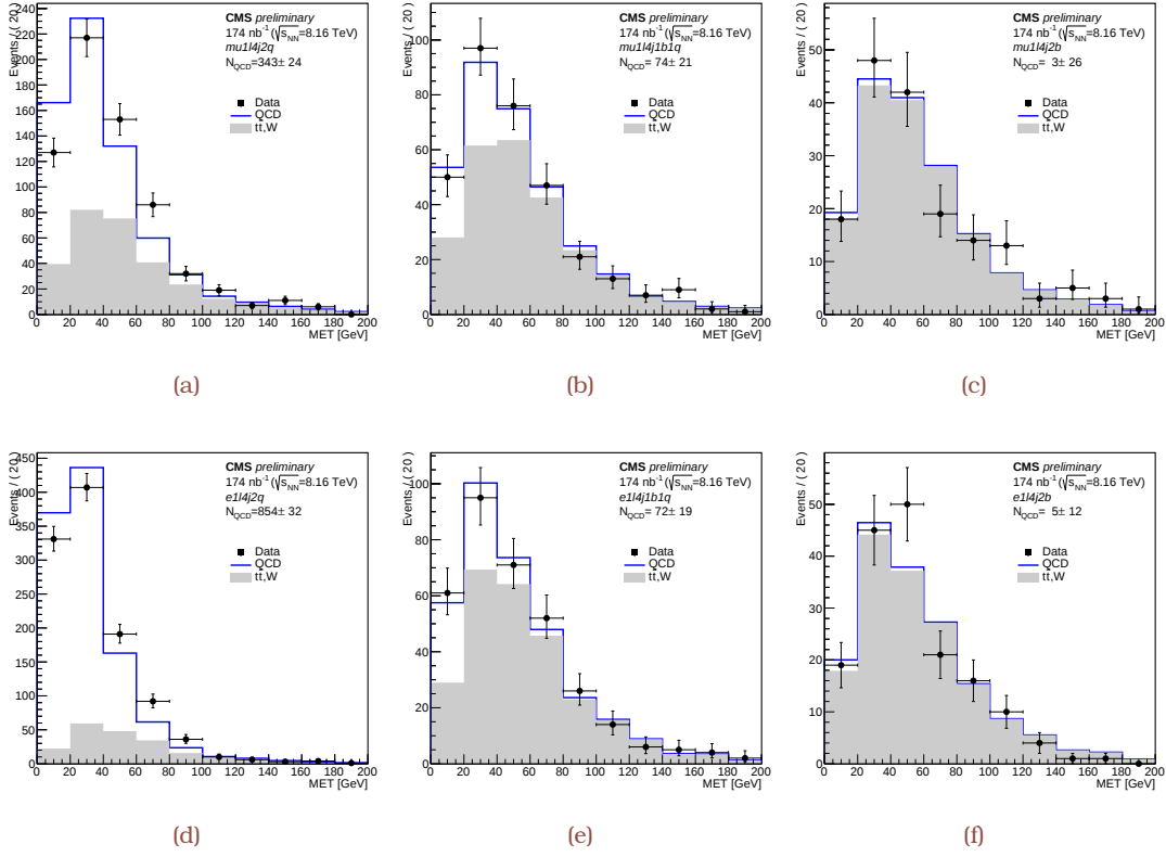
Figure 6.15: Fits to the p_T^{\text{miss}} distribution in the \mu +jets (a-c) and e +jets (d-f) final states in the 1\ell4j0b (a, d), 1\ell4j1b (b, e), and 1\ell4j2b (c, f) event categories. The QCD normalization estimated from the fit is shown in the captions, along with its statistical uncertainty [AN2].
