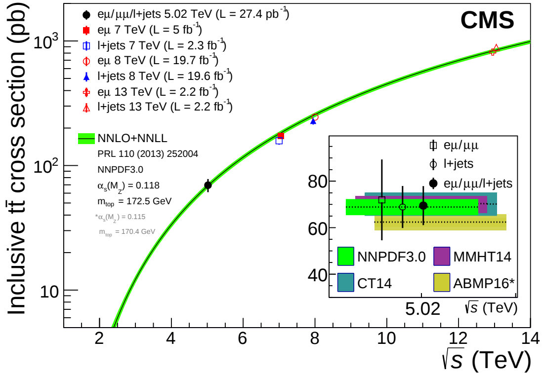
Figure 5.16: Inclusive \sigma_{t\bar{t}} in pp collisions as a function of the center-of-mass energy; previous CMS measurements at \sqrt{s} = 7, 8 [246, 247], and 13 [75, 250] TeV in the separate \ell +jets and dilepton final states are displayed, along with the combined measurement at 5.02 TeV from this analysis [TH4]. The NNLO+NNLL theoretical prediction [258] using the NNPDF3.0 [35] PDF set with \alpha_s(M_Z) = 0.118 and m_{t\text{top}} = 172.5 GeV is shown in the main plot. In the inset, additional predictions at \sqrt{s} = 5.02 TeV using the MMHT14 [34], CT14 [33], and ABMP16 [32] PDF sets, the latter with \alpha_s(M_Z) = 0.115 and m_{t\text{top}} = 170.4 GeV, are compared, along with the NNPDF3.0 prediction, to the individual and combined results from this analysis. The vertical bars and bands represent the total uncertainty in the data and in the predictions, respectively.
