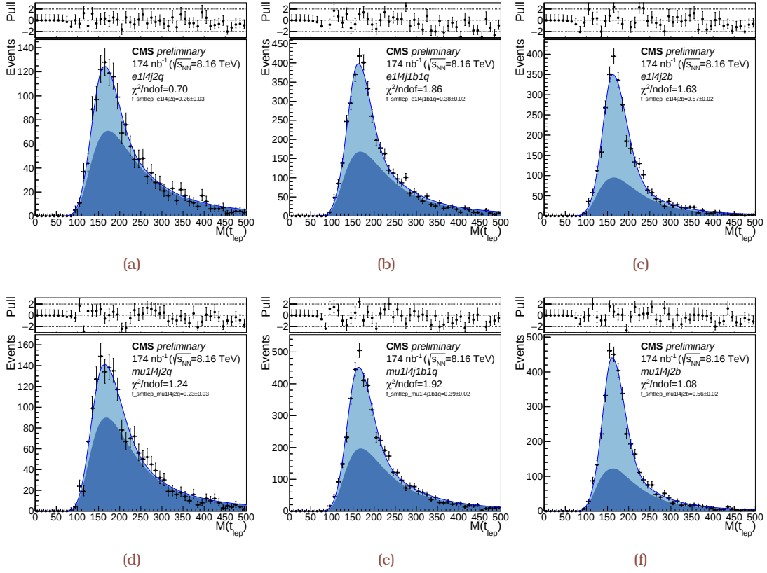
Figure 6.10: Parametrized signal spectra in e+jets (a–c) and \mu +jets (d–f) final states as a function of m_{t_{lep}} in the 1 \ell 4j0b (a, d), 1 \ell 4j1b (b, e), and 1 \ell 4j2b (c, f) event categories, using the PYTHIA MC simulation (Table 6.1). In the bottom panels, the estimated contributions from correct (wrong) assignments are shown in light (dark) blue. The parameterizations of correct and wrong assignments are fitted to the MC simulated events (points) and their difference, divided by the statistical uncertainty in the simulation, is represented on the top panels [AN2].
