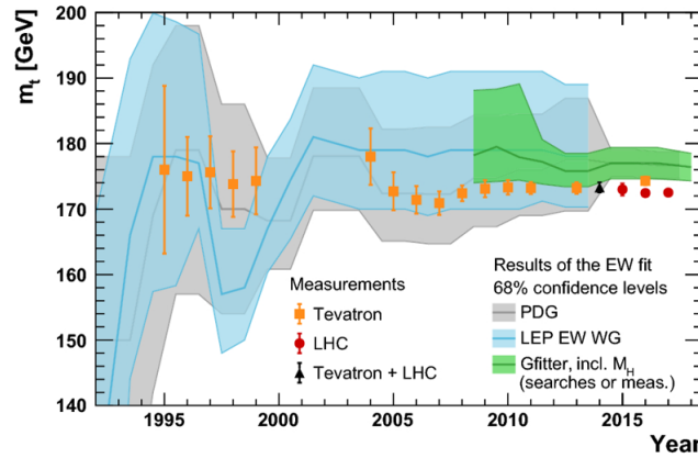
Figure 1.1: Prediction of the top quark mass as a function of time as obtained by various analysis groups using electroweak precision data. The bands indicate the 68% confidence level. The direct measurements after the top quark discovery are displayed by the data points [9]. The good agreement between the top quark mass measured directly and the predicted mass determined indirectly from measurements at the Z pole is a convincing illustration of the validity of radiative corrections.
