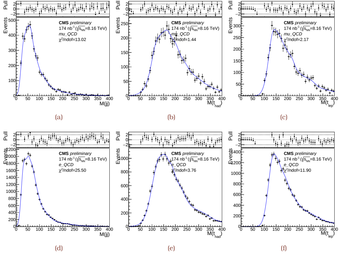
Figure 6.14: Parametrized QCD multijet distributions as a function of m_{jj'} (a), m_{t_{\text{had}}} (b) and m_{t_{\text{lep}}} (c) using events with no b-tagged jets in (a–c) \mu +jets—failing I_{\text{rel}}^\mu > 0.2 requirement—and (d–f) e +jets—failing the veto identification—final states, respectively [AN2].
