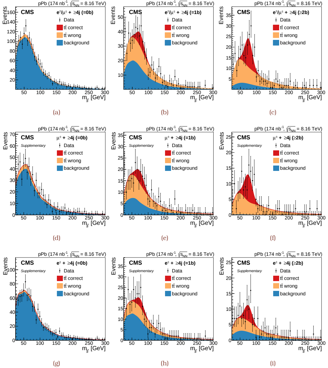
Figure 6.16: Invariant mass distributions of the W candidate, m_{j\ell} , in the 0 (a, d, g), 1 (b, e, h), and 2 (c, f, i) b-tagged jet categories after all selections in the \ell +jets (a–c), \mu +jets (d–f) and e +jets (g–i) final states. The red and orange areas correspond to the signal simulation (correct and wrong assignments, respectively) while the blue one corresponds to the estimated non-top background contributions. The error bars indicate the statistical uncertainty [TH1].
