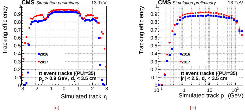
Figure 3.9: Track reconstruction efficiency—the number of reconstructed tracks sharing at least 75% of their assigned hits with the simulated particles divided by the total number of generated particles—as a function of the simulated track (a) \eta and (b) p_T [172]. The phase-I pixel detector (installed in 2017) exhibits an improved performance relative to the phase-0 detector all over the \eta and studied p_T spectrum. The reconstructed tracks are simulated based on PYTHIA (v.8 [50, 51]) using the 4C tune [174], and are required to meet the “high-purity” requirement (Table 3.1). The number of pileup interactions superimposed on each simulated t\bar{t} event is randomly generated from a Poisson distribution with a mean value of 35.
