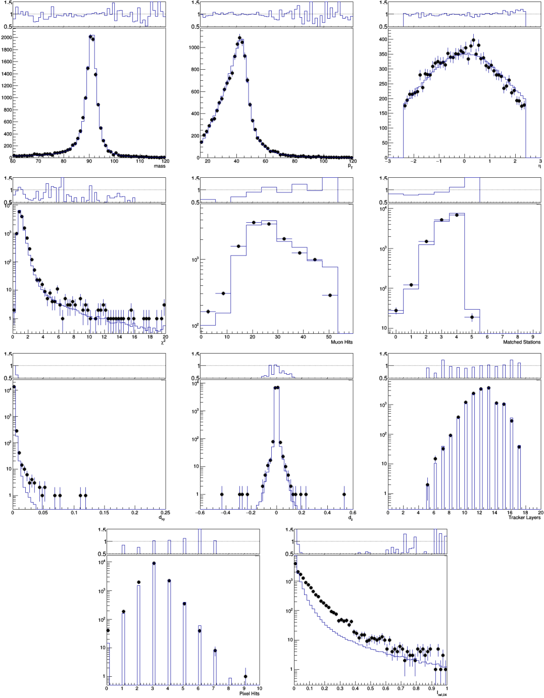
Figure 3.17: Muon kinematic (invariant mass, p_T , and \eta ) and identification variables for Z \rightarrow \mu\mu events at \sqrt{s_{NN}} = 8.16 TeV. Data (Table B.1) are found to be in good agreement with the MC (Table 6.1) simulation—scaled to the integral of data—in most of considered variables, except for the isolation due to the presence of the underlying event [AN2]. The slight mismodeling in |d_0| can be attributed to the non-simulated background and imperfect simulation of the tracker alignment.
