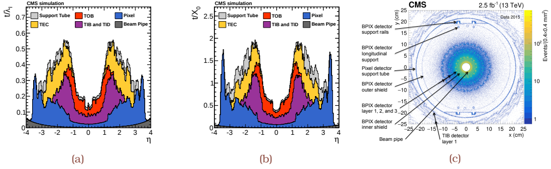
Figure 2.14: Total thickness t of the inner tracker material expressed in units of interaction (a) and radiation (b) lengths, l_i and X_0 , respectively, as a function of the pseudorapidity \eta [145]. (c) “Hadrography” is based on samples of secondary hadronic interactions and produces a high-precision map of the material within the tracking volume. The density of vertices is indicated by the color scale [146].
