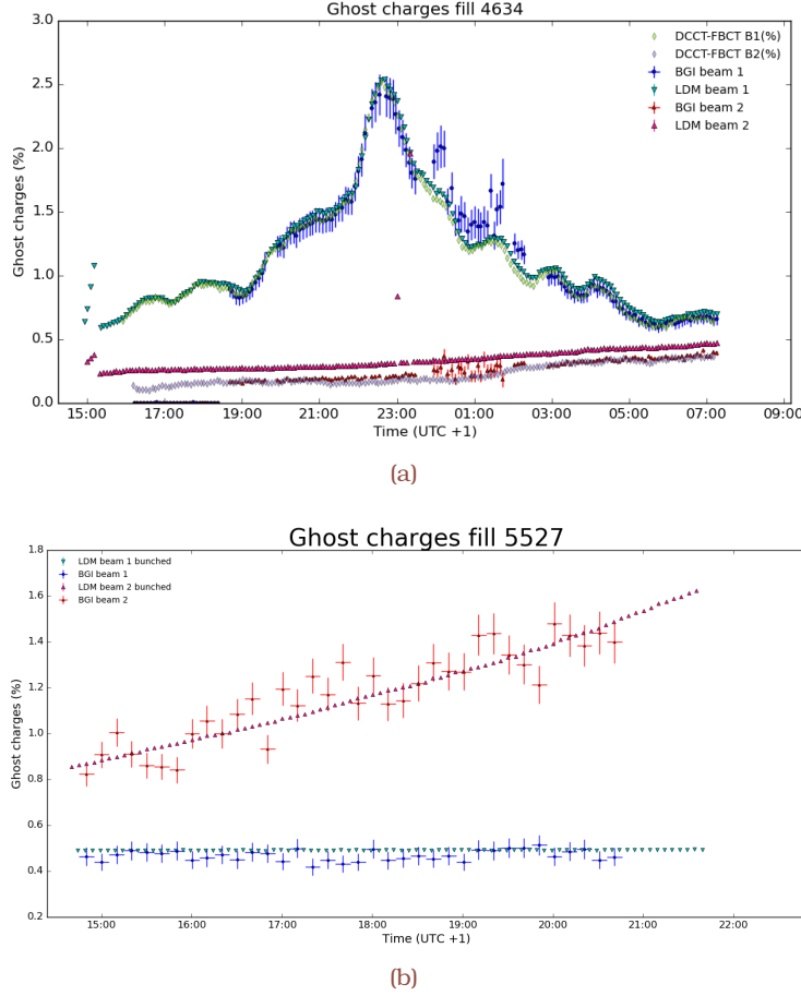
Figure 4.17: Ghost-charge fractions separately for beam 1 and 2 as a function of time for Fills 4634 (a) and 5527 (b) comparing the measurements based on the number of beam-gas interactions (BGI) recorded by LHCb [237] and the longitudinal profile of the synchrotron radiation monitors. The total systematic uncertainty in BGI measurements stems from the trigger efficiency that is fully correlated between the beams. The unbunched population, i.e., the signal level at RF edges, is not subtracted from LDM measurements. The FBCT—normalized to the first valid LHCb ghost-charge value per beam—is subtracted from the DCCT measurement and is superimposed in (a).
