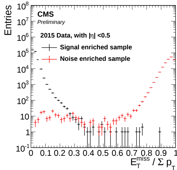
Figure 3.32: The distributions of the p_T^{\text{miss}} over the scalar p_T sum ( \sum p_T ) ratio in signal- and noise-enriched events using back-to-back dijet (black) and a minimum-bias selection without applying any PF jet identification requirements (red), respectively [191].
