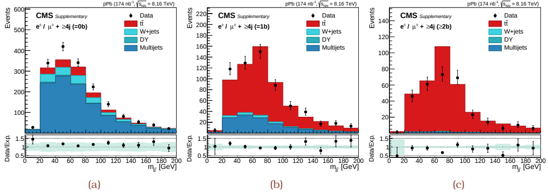
Figure 6.3: Dijet invariant mass ( m_{jj'} ) distributions in the 1l4j0b (a), 1l4j1b (b), and 1l4j2b (c) event categories after the complete event selection. On the upper panels, the reconstructed data are compared to the stacked expected contributions from the signal and the main background processes [TH1]. The t\bar{t} , W+jets, and Drell-Yan (DY) processes are simulated with PYTHIA (v6.424 [49], tune Z2* [58, 177]) and normalized to the theoretical cross sections (Table 6.1). The QCD multijet (Multijets) contribution is estimated from data using a control region. The bottom panels display the ratio between the data and the expectations. The shaded band represents the relative uncertainty due to the limited statistics in the simulated samples and in the estimate of the normalization of the QCD multijet background.
