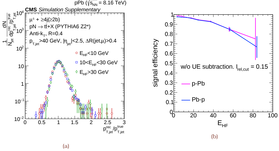
Figure 3.15: (a) Jet energy scale for jets in simulated t\bar{t} events using pPb collisions at \sqrt{s_{NN}} = 8.16 TeV. Reconstructed jets overlapping with the isolated muon are excluded [TH1]. (b) The efficiency loss due to the muon isolation as a function of the energy in the HF subdetector. Similar conclusions are drawn for electrons [AN2].
