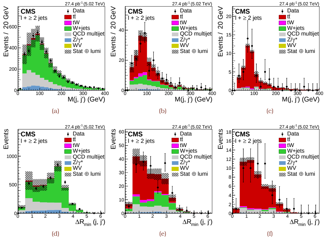
Figure 5.12: The predicted and observed distributions of the (a–c) M(j, j') and (d–f) \Delta R_{\min}(j, j') variables for \ell + \text{jets} events in the 0b (a,d), 1b (b,e), and \geq 2b (c,f) tagged jet categories. The distributions from data are compared to the sum of the expectations for the signal and backgrounds prior to any fit. The QCD multijet background is estimated from data (see Section 5.4.1). The cross-hatched band represents the statistical and the integrated luminosity uncertainties in the expected signal and background yields added in quadrature. The vertical bars on the data points represent the statistical uncertainties [TH4].
