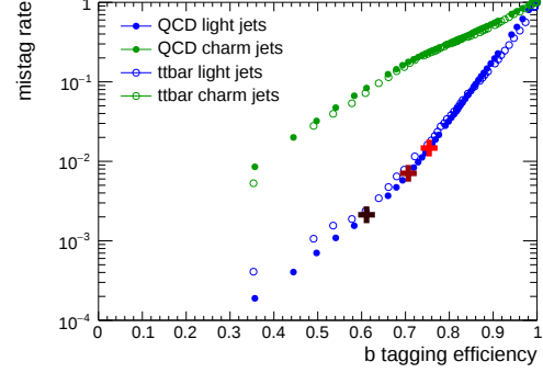
Figure 3.28: Misidentification probability for c and light-flavor jets against b jet identification efficiency in pPb collisions at \sqrt{s_{NN}} = 8.16 TeV separately determined from t\bar{t} and QCD multijet simulations [AN2].
