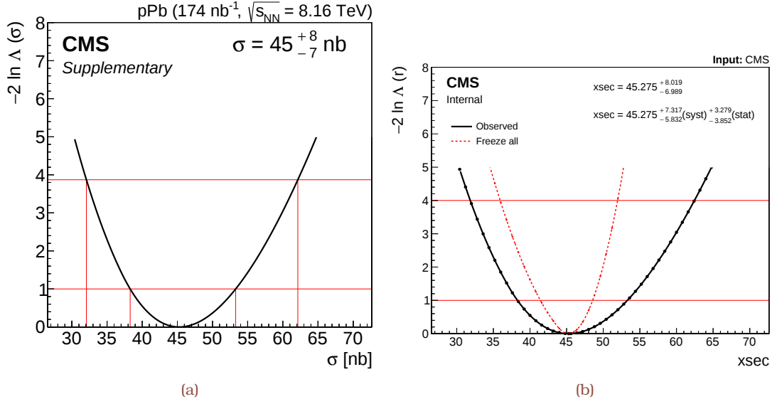
Figure 6.18: Profile likelihood ratio variation as a function of the parameter of interest for the nominal m_{t\bar{t}} analysis corresponding to the (a) total [TH1] and (b) split into statistical and systematic uncertainties [AN2]. The two horizontal lines on (a) represent the values in the profile likelihood that are used to determine the 68 and 95% confidence level intervals for the \sigma_{t\bar{t}} .
