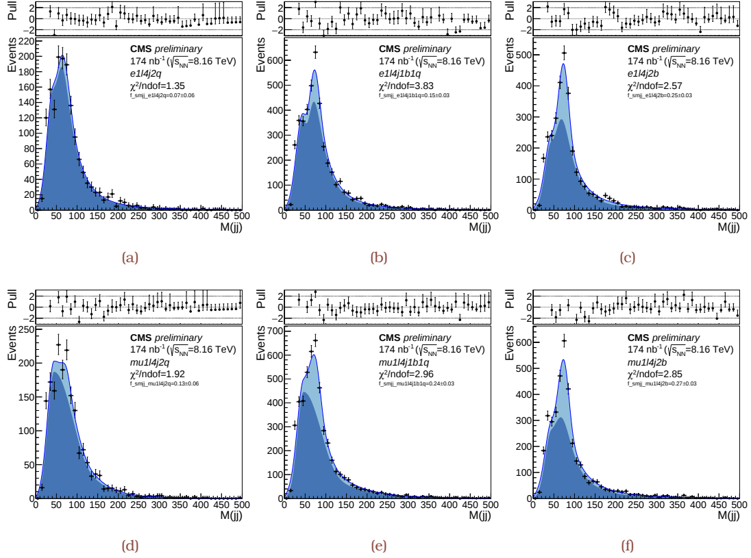
Figure 6.8: Parametrized signal spectra in e +jets (a-c) and \mu +jets (d-f) final states as a function of m_{jj} in the 1l4j0b (a, d), 1l4j1b (b, e), and 1l4j2b (c, f) event categories, using the PYTHIA MC simulation (Table 6.1). On the bottom panels, the estimated contributions from correct (wrong) assignments are shown in light (dark) blue. The parameterizations of correct and wrong assignments are fitted to the MC simulated events (points) and their difference, divided by the statistical uncertainty in the simulation, is represented on the top panels [AN2].
