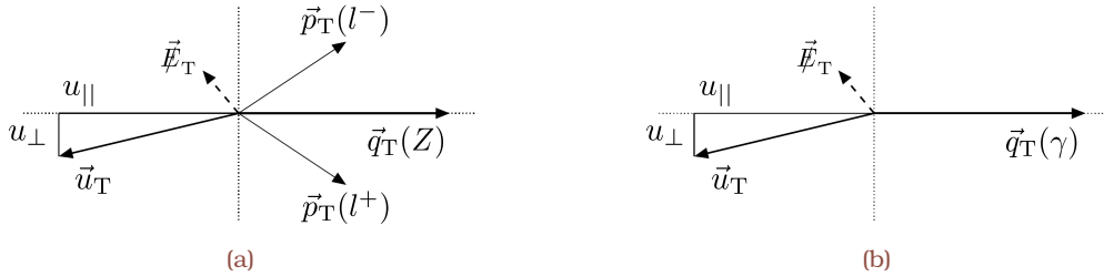
Figure 3.30: Illustration of the Z/ \gamma^* (a) and photon (b) event kinematics in the transverse plane. The vector \vec{u}_T denotes the vector p_T sum of all particles reconstructed in the event excluding the two leptons from the Z/ \gamma^* decay or the photon [189].
