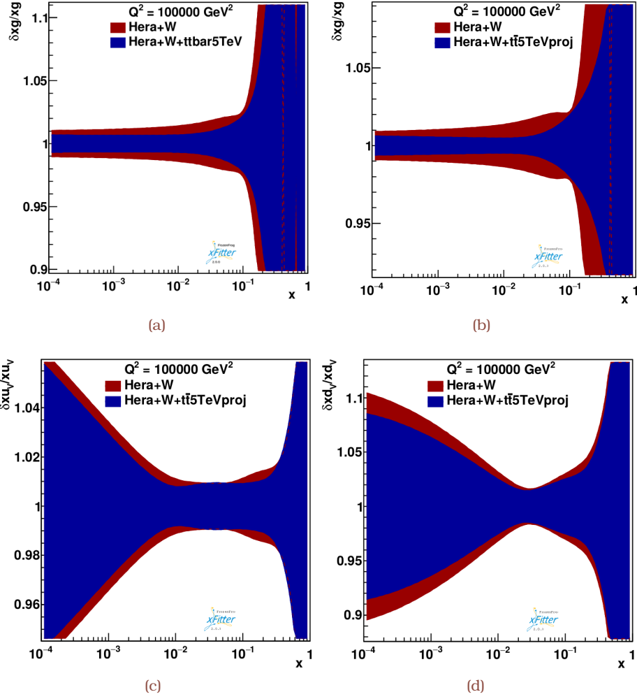
Figure 7.4: (a) The relative uncertainties in the gluon distribution functions of the proton as a function of x at \mu_F^2 = 10^5 \text{ GeV}^2 from a QCD analysis using the HERA DIS and CMS muon charge asymmetry measurements, and also including the CMS \sigma_{\text{ti}} results at \sqrt{s} = 5.02 \text{ TeV} . (b) Same as (a) but corresponding to the conjectured \sigma_{\text{ti}} results. (c, d) Same as (b) but corresponding to the relative uncertainties in the valence quark distribution functions. The latter needs to be compared with Figs. 5.18d and 5.18d, respectively.
