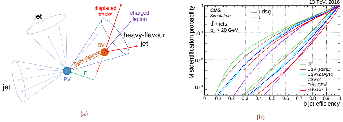
Figure 3.26: (a) Illustration of a heavy-flavor jet with a secondary vertex (SV) from the decay of a b hadron [201]. The displacement of tracks, including possibly an identified lepton, with respect to the primary interaction vertex is characterized by their impact parameter (IP). The IP can receive both positive and negative values, with a positive sign indicating that the track is produced “upstream,” namely, the angle between the impact parameter vector and the jet axis is less than \pi/2 . (b) Misidentification probability for c and light-flavor jets against b jet identification efficiency [201].
