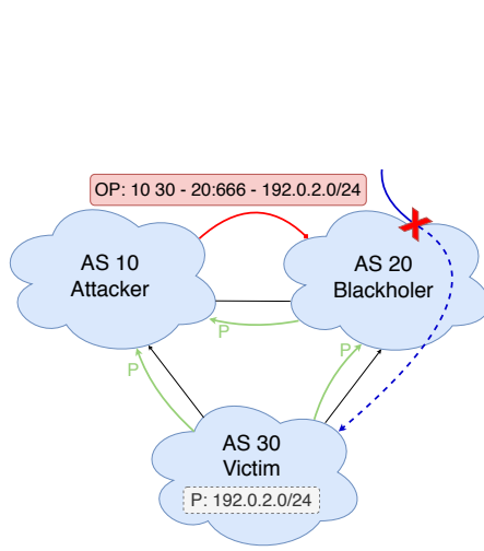
Fig. 4: On Path Blackjack
