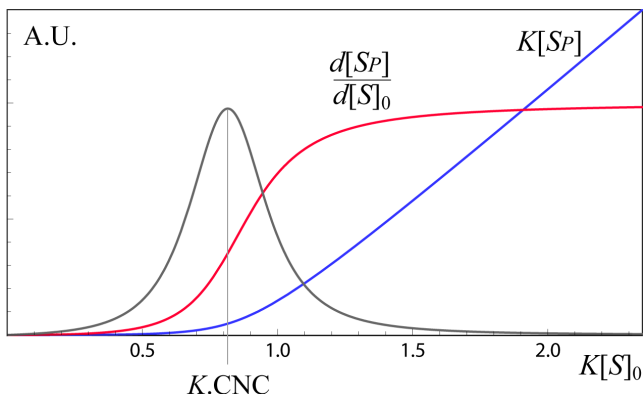
Figure 1 Representation in arbitrary units of the accumulation of aggregates (blue curve), its derivative (red curve) and its curvature (grey curve) as functions of the total concentration of subunits. The nucleation parameters used are n = 3 and F_3 = 0.004 . The curvature is used to determine the critical nucleation concentration, as defined in (34), over which aggregates significantly accumulate. K is the binding constant of polymerization.
