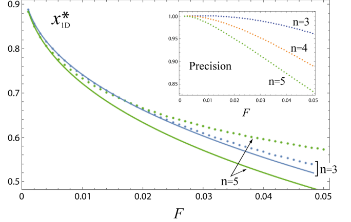
Figure 2 Comparison, for the 1D models, between the exact numerical results (dotted) and those obtained from the series (36) (continuous line) for the point x_{1D}^* of maximal curvature, defining the CNC. The blue and green curves are for n=3 and n=5 respectively. The inset shows the level of precision as a function of F (the data shown are the absolute values of the ratios of x_{1D}^* computed from the truncated series to its exact numerical value).
