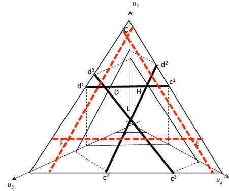
Fig 14: A game where the ISI set (CEF) contains the \gamma -core (DHL)
