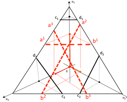
Fig. 10 A game where the ISI set is empty.
