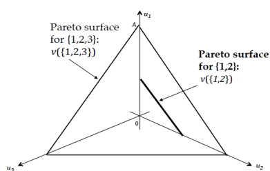
Fig. 2 What coalition \{1,2\} can do
