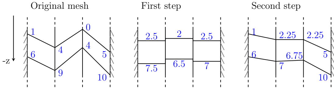
Fig. 5: Illustration of the horizontal smoothing algorithm on a 2D “ x - z ” mesh. First, for each element, the upper and lower nodal values of the vertical coordinate z are set to their mean value, then z is projected onto a continuous field. The numbers refer to the depth of the mesh levels.
