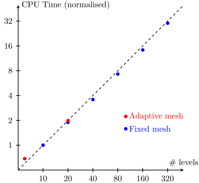
Fig. 11: CPU time of the simulations for a different number of levels (using a loglog scale). CPU time are normalised by the 10 fixed levels simulation time. As expected, CPU time is proportional to the number of levels. Moreover, the computational overhead of adaptive levels is negligible. For the same computational cost, the adaptive method is then much more accurate (Fig. 10).
