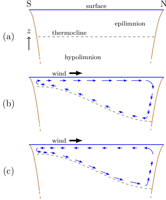
Fig. 2: Schematic lake configuration with no wind stress (a) and with the south-easterly wind during the dry season in line with the classical circulation (b, Mortimer, 1961) such that the surface water follows the wind, or according to the non-classical circulation (c, Verburg et al., 2008) with reversed currents.
