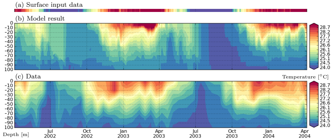
Fig. 15: Lake water temperature (°C) at Mpulungu as predicted by the model (b) and from in situ observations (c, Descy et al., 2006). Panel (a) shows the surface temperature used to force the temperature flux at the lake surface (Thiery et al., 2015).
