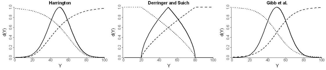
Figure 1: Different desirability functions. The continuous lines represent cases of a targeted property and the dotted and dashed lines represent cases of a minimized and a maximized property respectively.
