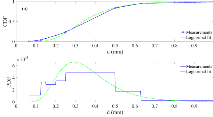
Figure 2. (a) Cumulative Density Function (CDF) and (b) Probability Density Function (PDF) of the sand used in the experiments. The CDF was interpolated with a step of 1 \text{ } \mu\text{m} to derive the PDF. The few sieves used to establish the CDF explain the stepped appearance of the PDF. The lognormal fit uses \mu_{\log} = \log(0.5d_{50}/\sqrt{1+\delta^2}) and \sigma_{\log} = \sqrt{\log(\delta^2 + 1)} as distribution parameters, following Thorne & Hurther (2014), with \delta = 0.4 .
