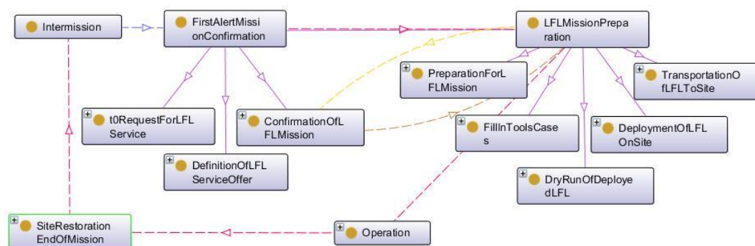
Figure 3. Fragment of ontology showing a few links between operational functions in the cycle FirstAlertAndMissionConfirmation, and LFLMissionPreparation.
