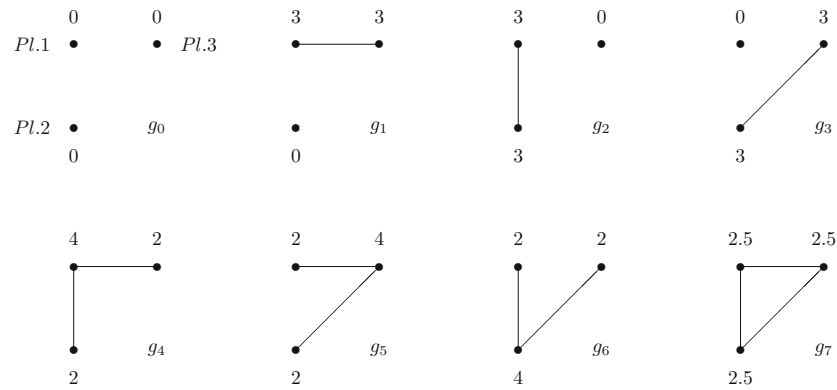
Fig. 1 The co-author model with three players
