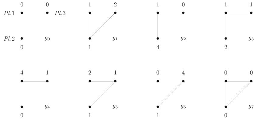
Fig. 3 Non-existence of myopic-farsighted stable sets
