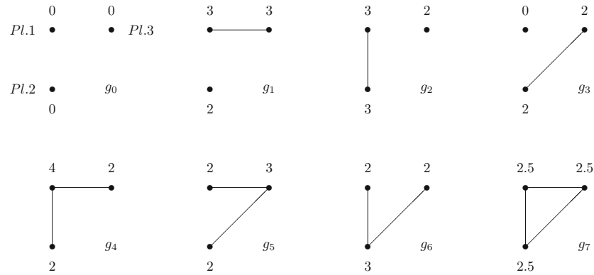
Fig. 2 A network formation game among three players
