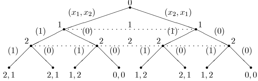
Figure 6: The extensive-form game for the social environment of Example 3.
