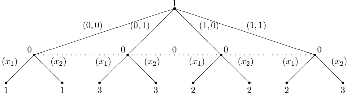
Figure 5: The extensive-form game for the social environment of Example 1.
