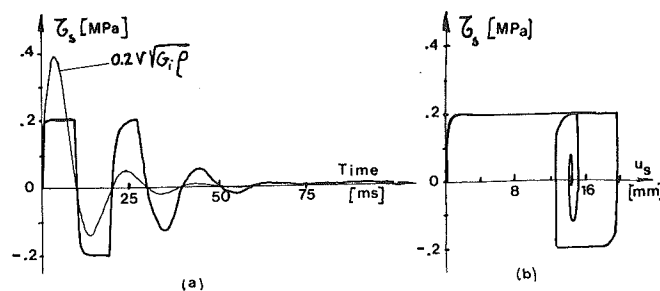
Fig. 8 : (a) Stress-time diagram (b) Stress-displacement diagram
