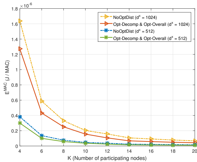
FIGURE 8: E^{\text{MAC}} vs. K for d^y = 1024 bits, N^{\text{LAY}} = 3 and \tau = 1 s
