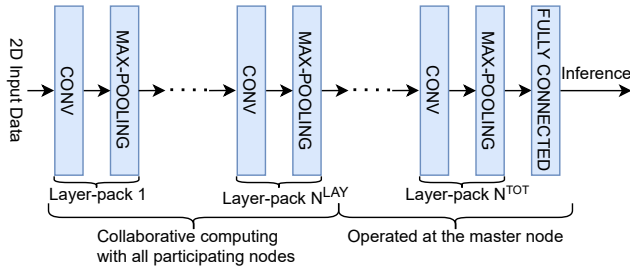
FIGURE 1: CNN model
