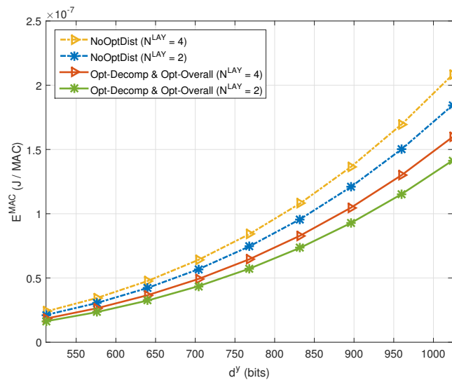
FIGURE 9: E^{\text{MAC}} vs. d^y for d^x = 512 bits, K = 10 and \tau = 0.5 s
