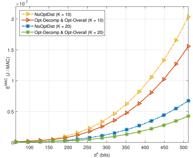
FIGURE 7: E^{\text{MAC}} vs. d^x for d^y = 1024 bits, N^{\text{LAY}} = 3 and \tau = 0.5 s
