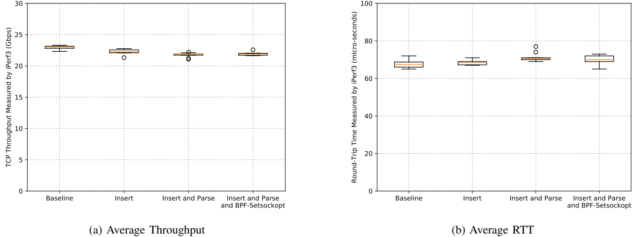
Fig. 4: Overhead of BPF-based TCP Option Operations in 3 cases vs. Baseline. iPerf3 client and server are on the same host, connected via loopback interface.
