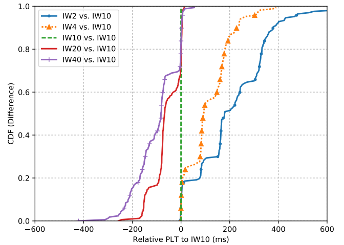
Fig. 6: Initial Window Option test: Page Load Time relatively to IW=10 (40 Mbps bandwidth, 40 ms link delay)
