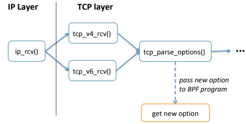
Fig. 3: Pass unknown TCP options of incoming packets to BPF program
