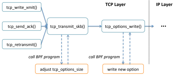
Fig. 2: Insert TCP options to outgoing packets
