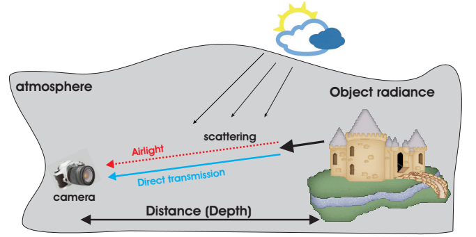
Fig. 2. Physical model of a hazy scene.
