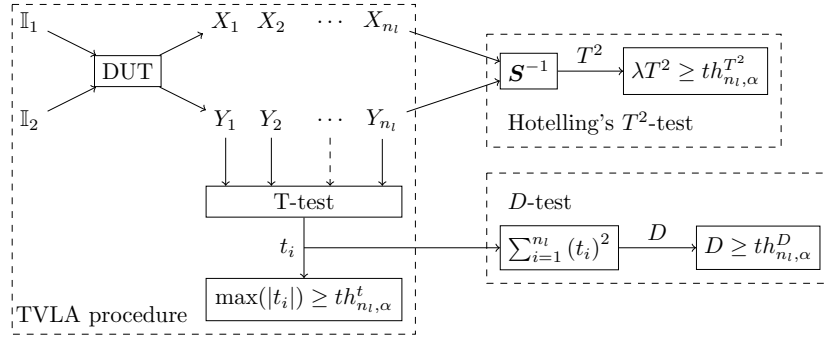
Figure 1: Leakage detection framework.
