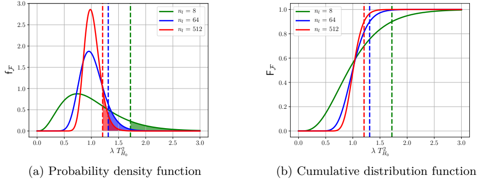
Figure 3: The PDF and CDF of different Fisher distributions with varying n_l and their corresponding threshold th_\alpha^{T^2} (dashed lines) for \alpha = 0.1 and N_{\mathbf{X}} = N_{\mathbf{Y}} = 64 .
