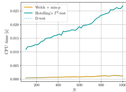
(b) n_l = 200
