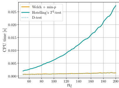
(a) N = 1000
