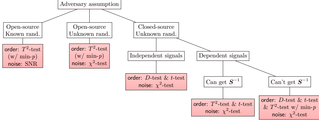
Figure 12: Proposed security assessment framework.
