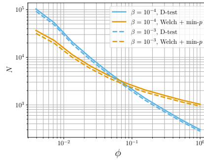
Figure 6: Number of traces N required to detect for a fixed false negative rate \beta on simulated traces with SNR = 0.01, and varying density \phi .
