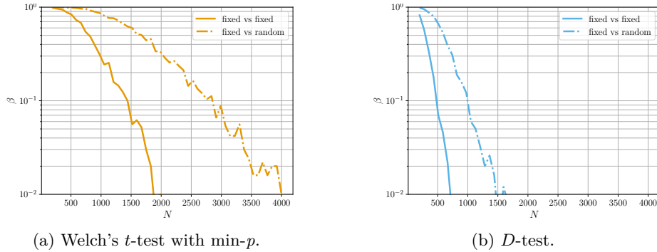
Figure 14: Detection rate for various input sets.
