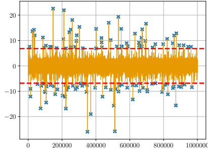
(a) Welch's t -tests' results obtained from pre-processed traces with N = 100,000 .
