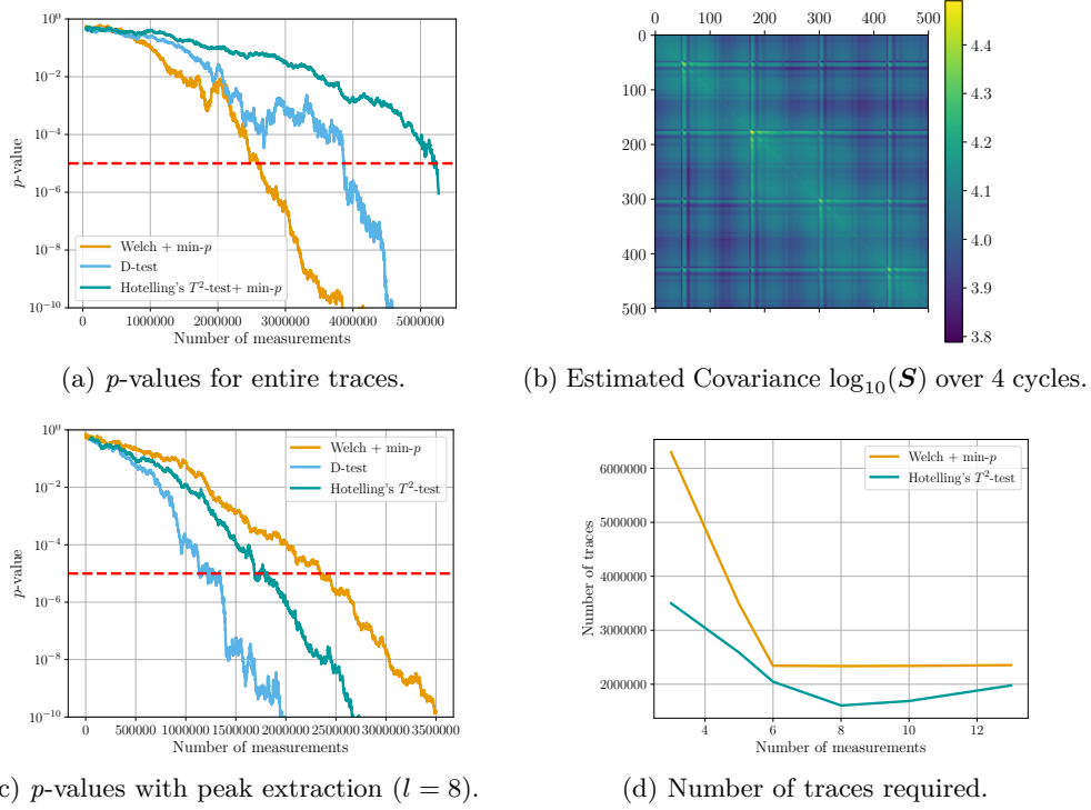
Figure 10: Leakage detection results using the measurements of a masked hardware AES implementation protected by DOM with two shares.
