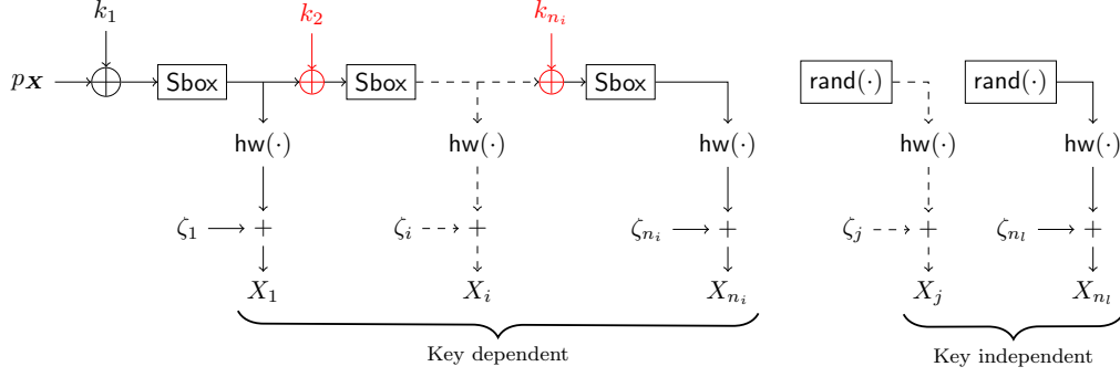
Figure 4: Simulation framework.
