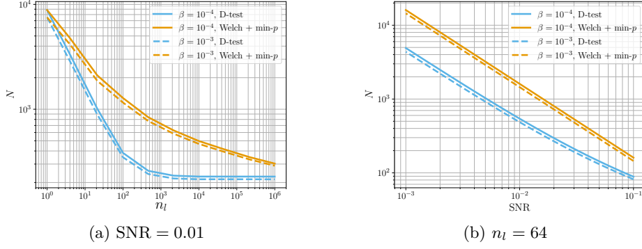
Figure 5: Number of traces N required to detect for a fixed false negative rate \beta on simulated traces with a density of \phi = 1 , and varying trace length n_l and SNR.
