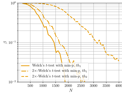
Figure 15: Detection rate of comparison with TVLA
